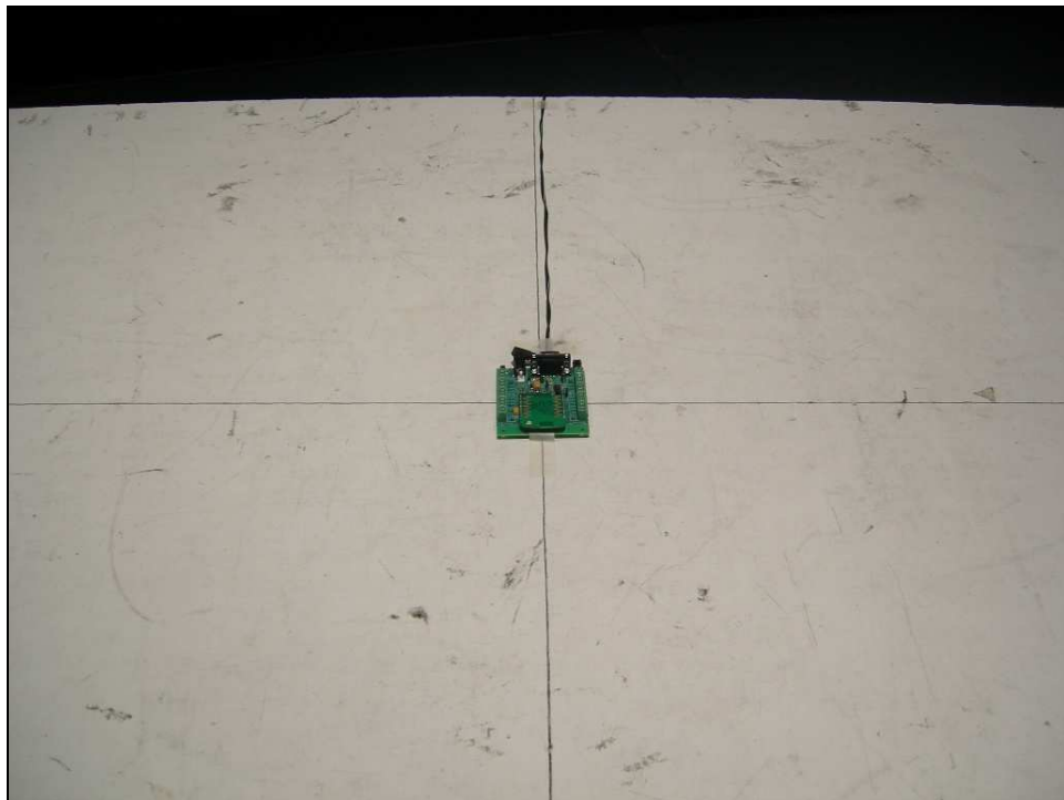
Figure 1: Radiated Emissions – Chip Antenna – Front View
