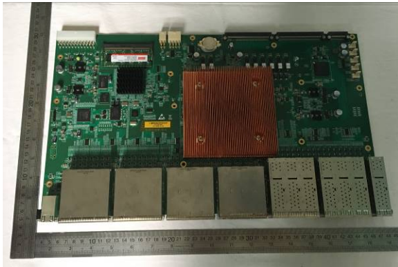
EUT –PCB View
