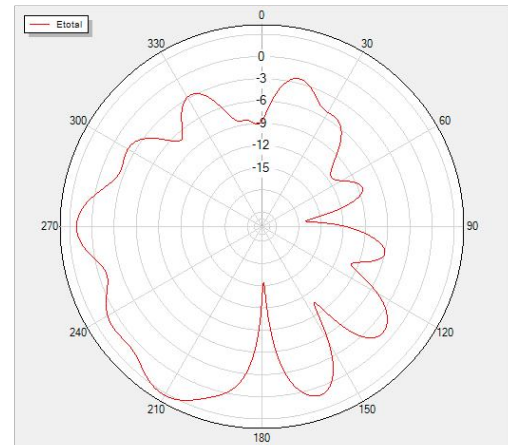
Phi=0 Freq=2440MHz
