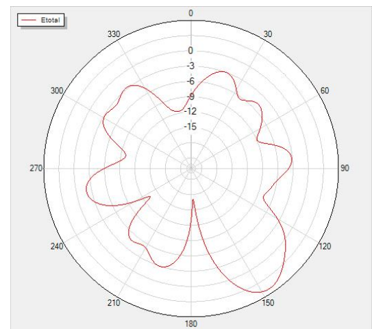
Phi=90 Freq=2440MHz
