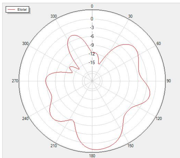
Theta=90 Freq=2440MHz
