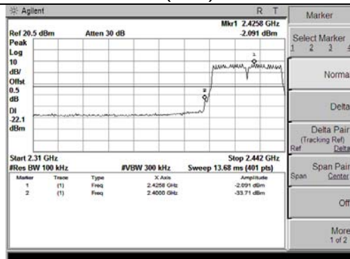
802.11 n(40M) Mode
