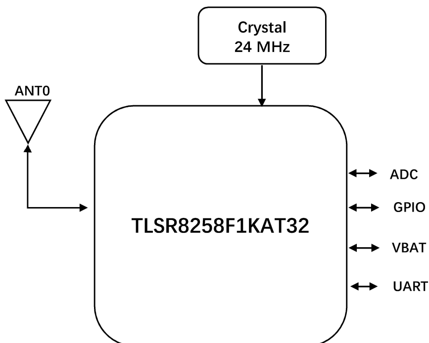
Fig 1 EWN-8258FAT1CA1 System Block Diagram
