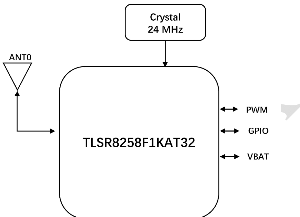
Fig 1 EWN-8258FAT1HA1 System Block Diagram
