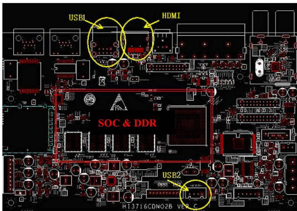
Fig 15 Main chip and DDR interference
