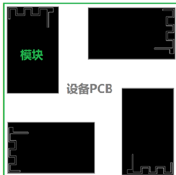
Fig 12 Recommended PCB layout
