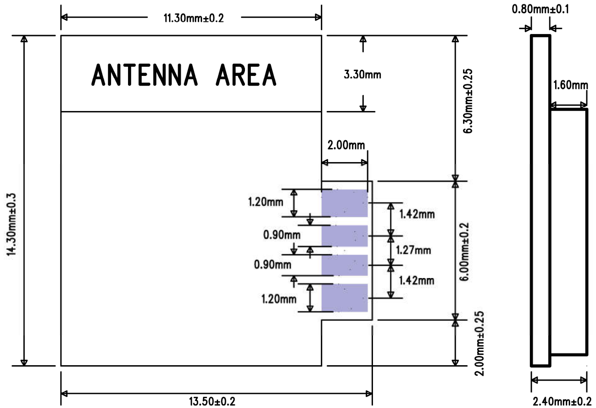
Fig 2 EWN-8258FAT1HA1 Top View Module Size
