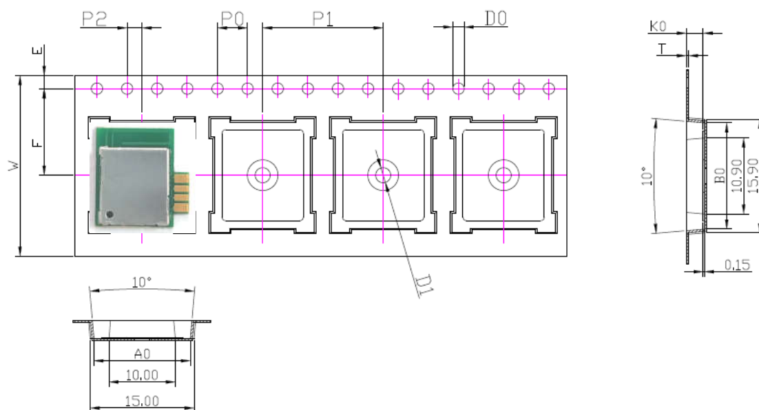
FIG 8 Carrier size
