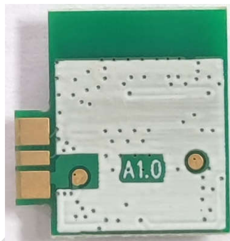
Fig 7 Bottom View
