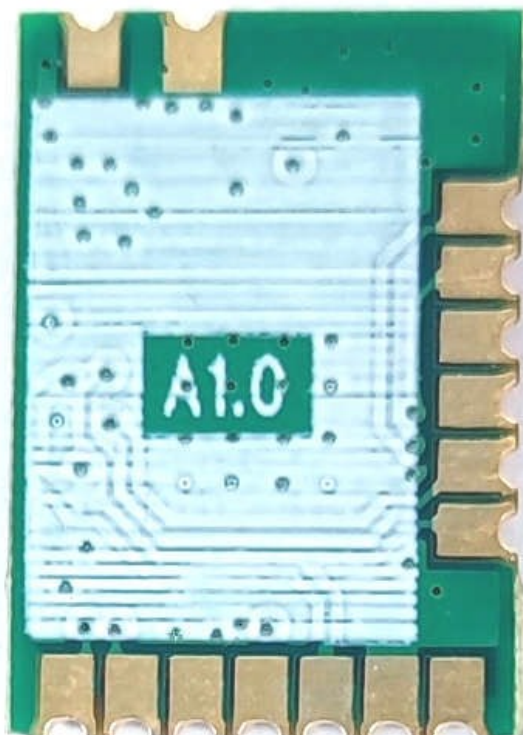
Fig 5 Bottom View
