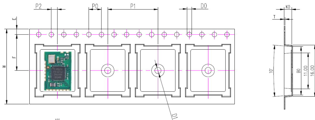
FIG 6 Carrier size
