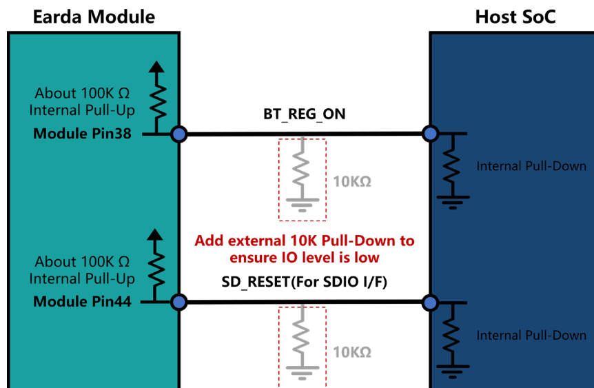
FIG 21 Add external pull down resistor to ensure low level
