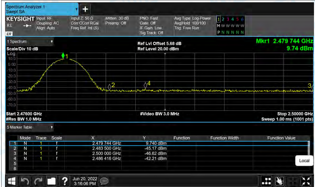
Restrict Band NVNT 2-DH1 2480MHz Ant1 No-Hopping Average
