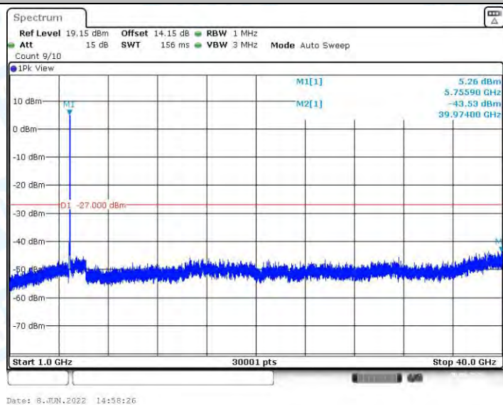
11AC40MIMO_Ant1_5755_1000~40000
