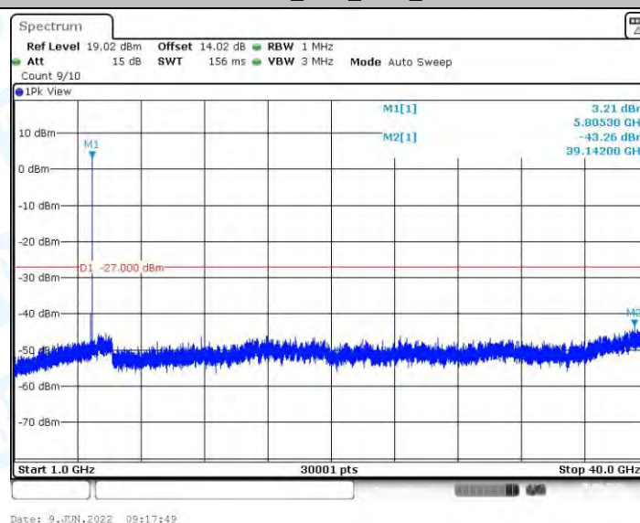
11AC80MIMO_Ant1_5775_1000~40000
