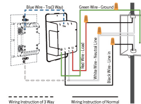
Wiring Instruction of 3 Way Wiring Instruction of Normal
