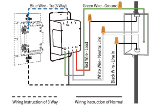
Wiring Instruction of 3 Way Wiring Instruction of Normal
