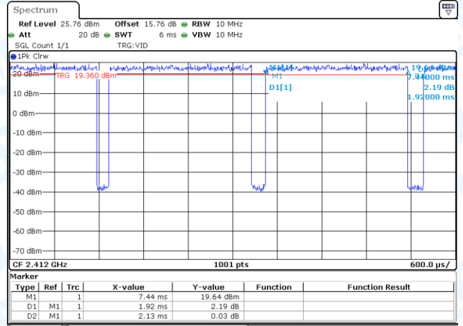
NTNV-11N20-CDD-Ant2-2412
