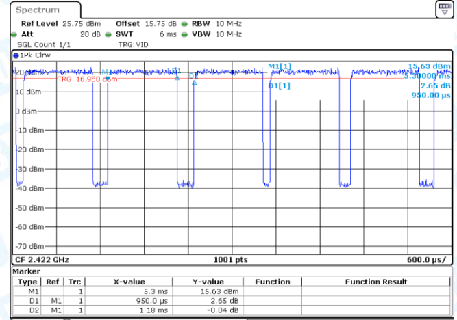
NTNV-11N40-CDD-Ant2-2422
