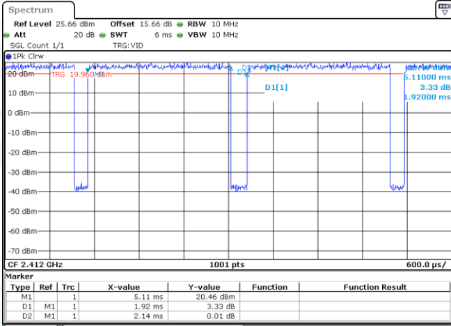
NTNV-11N20-CDD-Ant1-2412
