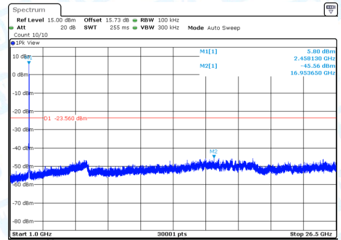
11N20-CDD-Ant2-2462-0~Reference-PASS
