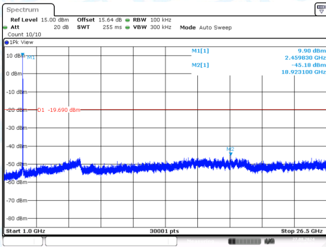
11B-Ant1-2462-0~Reference-PASS
