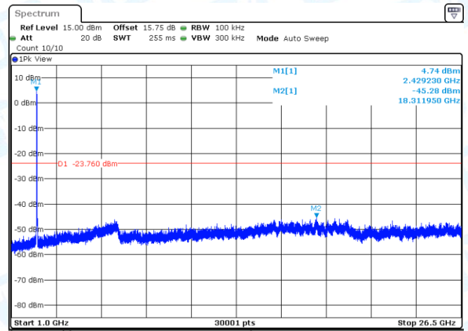
11G-Ant2-2437-0~Reference-PASS
