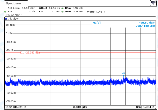
11N20-CDD-Ant1-2437-30~1000-PASS
