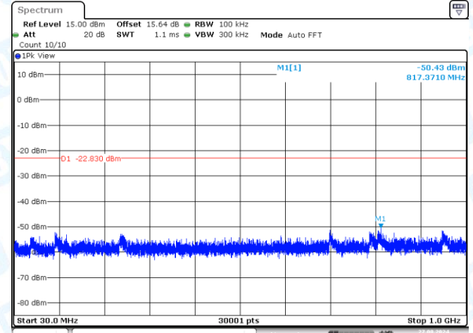
11N20-CDD-Ant1-2462-30~1000-PASS
