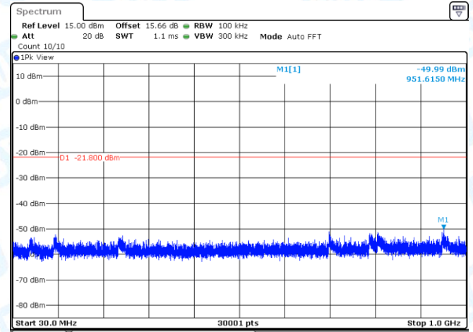
11N20-CDD-Ant1-2412-30~1000-PASS
