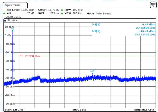
11G-Ant2-2462-0~Reference-PASS
