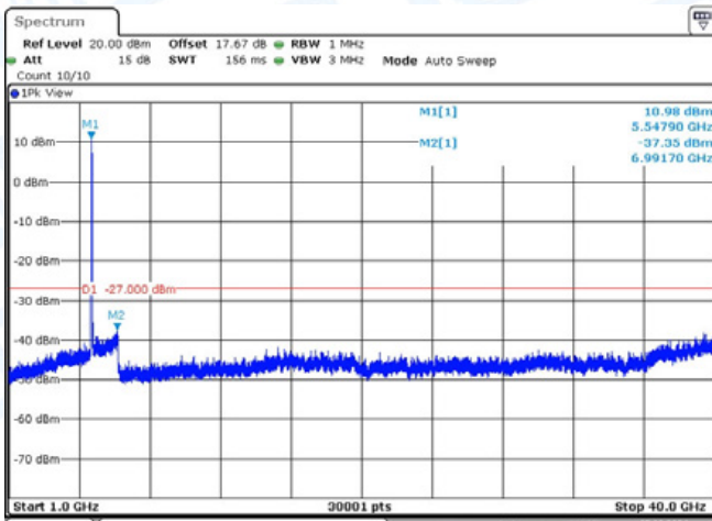
11AC40-CDD-Ant1-5550-1000~40000-PASS
