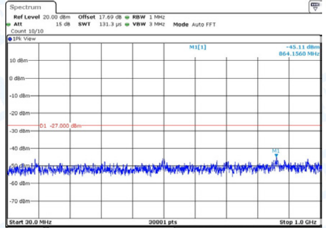
11AC40-CDD-Ant1-5795-30~1000-PASS
