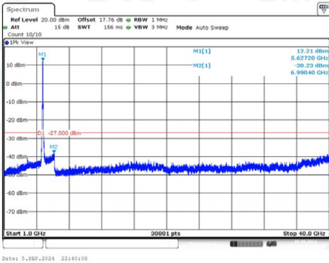
11AC80-CDD-Ant2-5610-1000~40000-PASS
