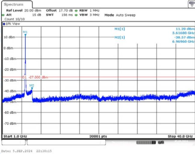
11AC80-CDD-Ant1-5610-1000~40000-PASS
