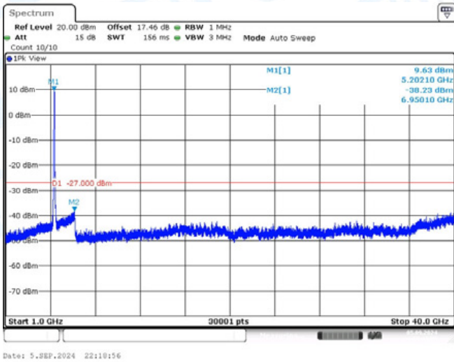
11AC80-CDD-Ant2-5210-1000~40000-PASS
