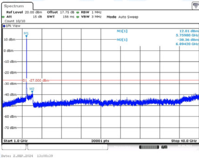
11AC40-CDD-Ant1-5755-1000~40000-PASS
