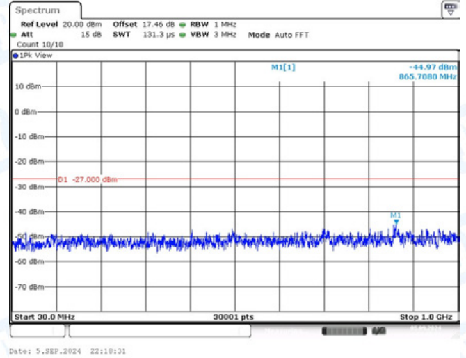
11AC80-CDD-Ant2-5210-30~1000-PASS
