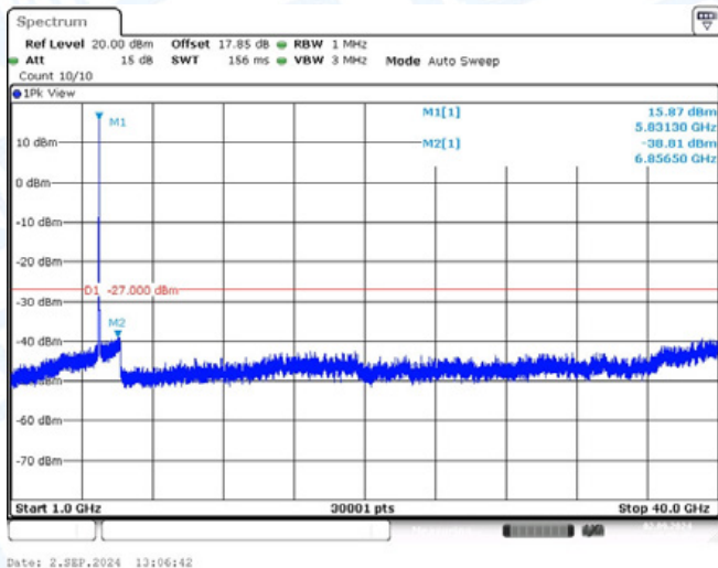
11AC20-CDD-Ant2-5825-1000~40000-PASS
