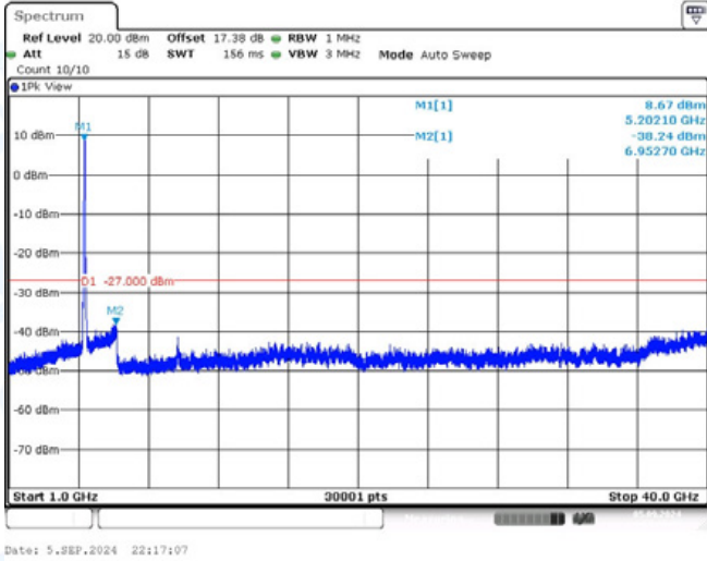
11AC80-CDD-Ant1-5210-1000~40000-PASS
