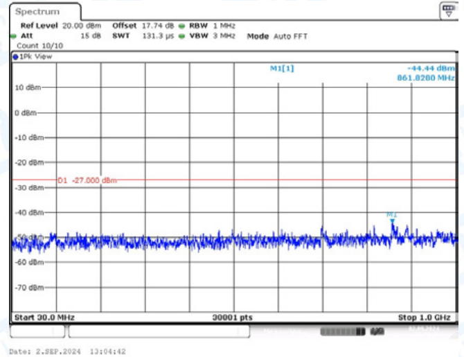
11AC20-CDD-Ant1-5825-30~1000-PASS
