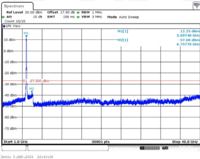
11AC80-CDD-Ant1-5690-1000~40000-PASS
