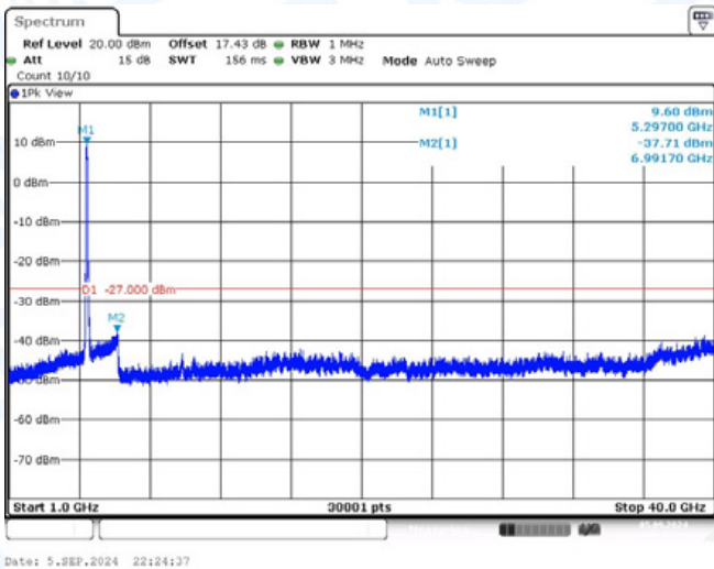
11AC80-CDD-Ant1-5290-1000~40000-PASS
