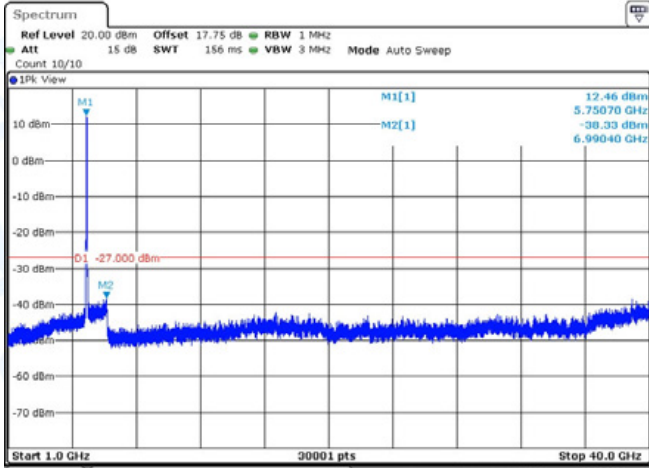
11AC40-CDD-Ant2-5755-1000~40000-PASS
