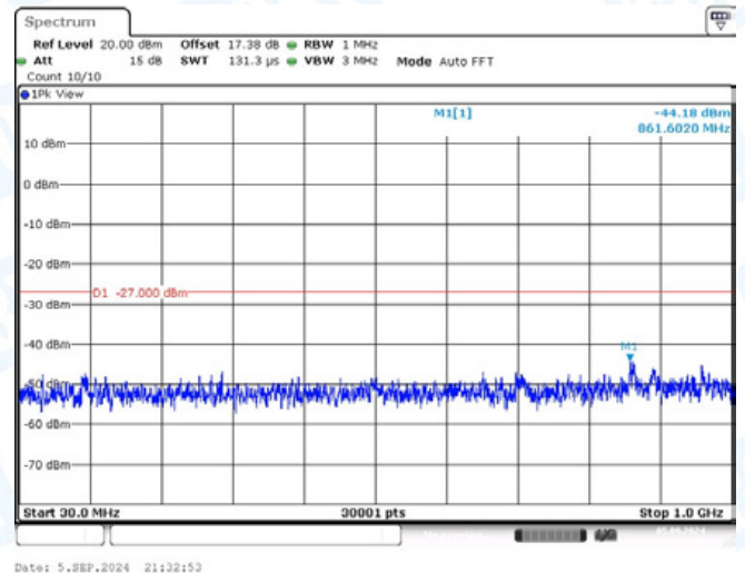
11AC40-CDD-Ant1-5190-30~1000-PASS
