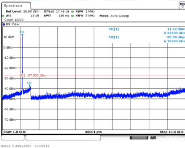
11AC40-CDD-Ant1-5230-1000~40000-PASS
