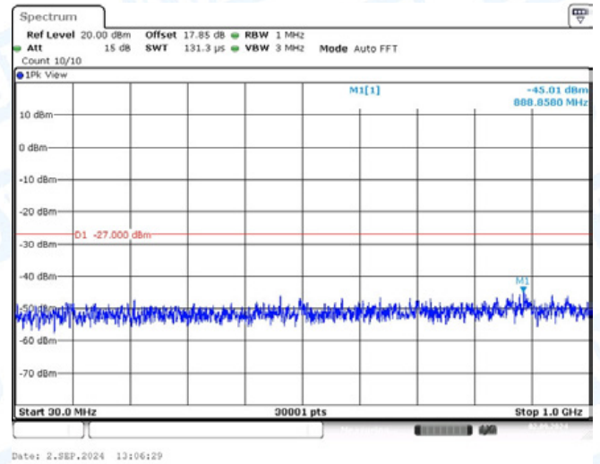
11AC20-CDD-Ant2-5825-30~1000-PASS
