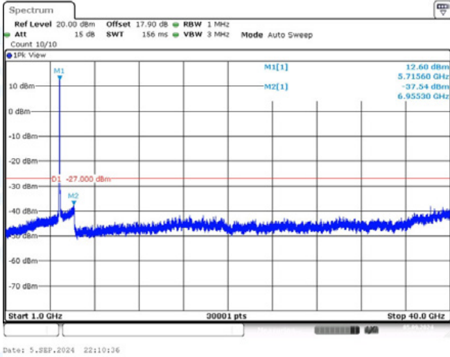
11AC40-CDD-Ant1-5710-1000~40000-PASS
