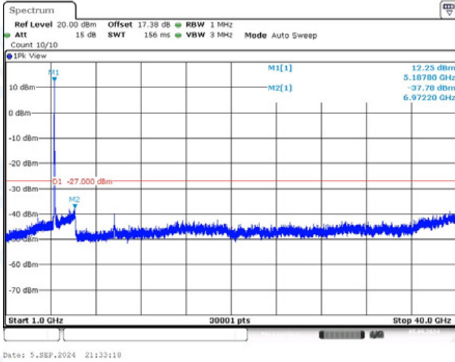
11AC40-CDD-Ant1-5190-1000~40000-PASS
