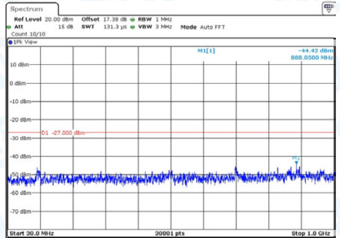
11AC40-CDD-Ant2-5795-30~1000-PASS
