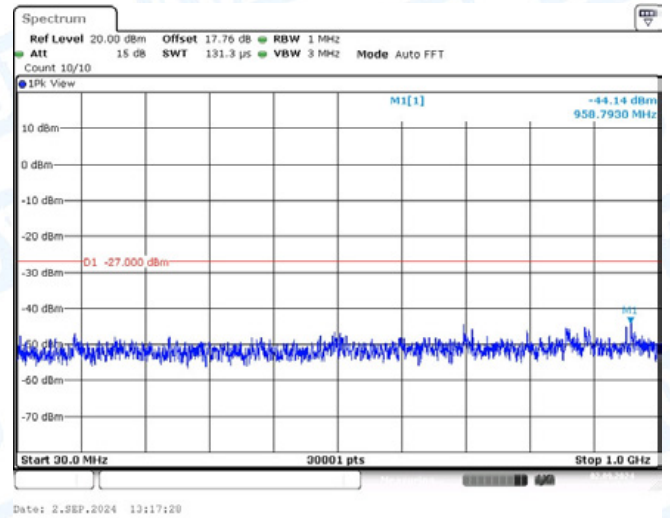
11AC80-CDD-Ant2-5775-30~1000-PASS
