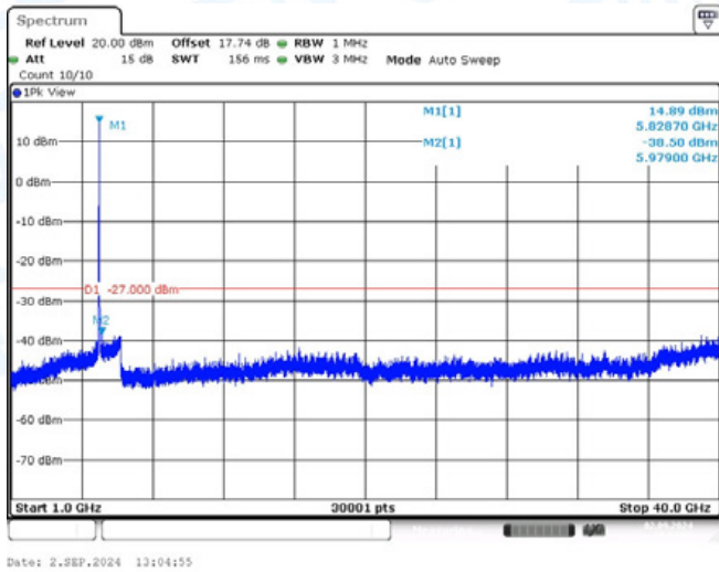
11AC20-CDD-Ant1-5825-1000~40000-PASS
