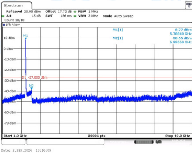
11AC80-CDD-Ant1-5775-1000~40000-PASS
