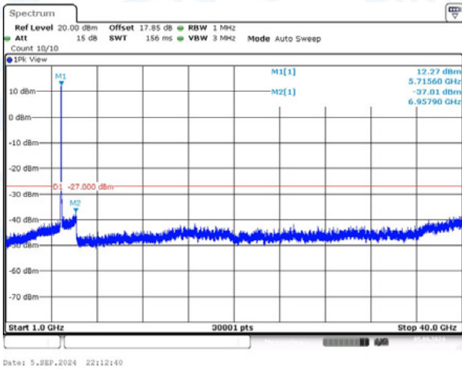
11AC40-CDD-Ant2-5710-1000~40000-PASS
