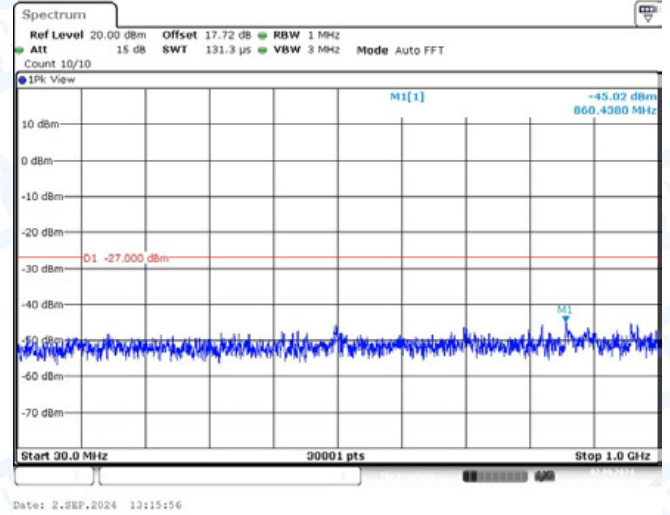
11AC80-CDD-Ant1-5775-30~1000-PASS
