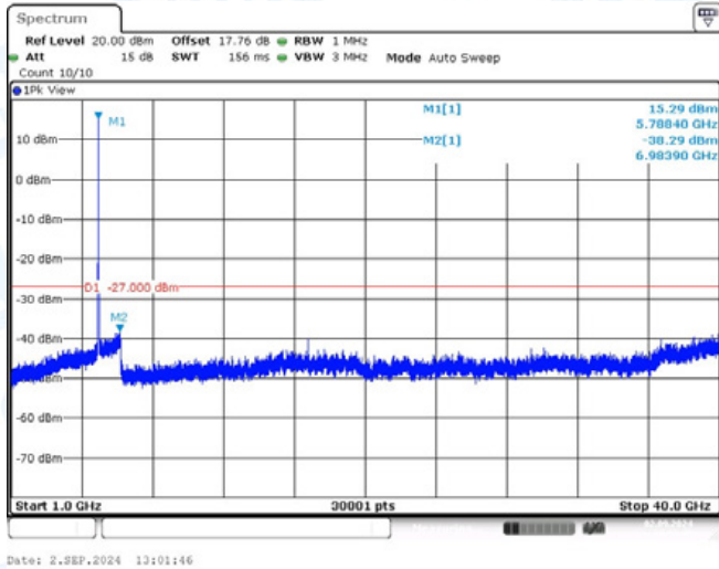
11AC20-CDD-Ant2-5785-1000~40000-PASS
