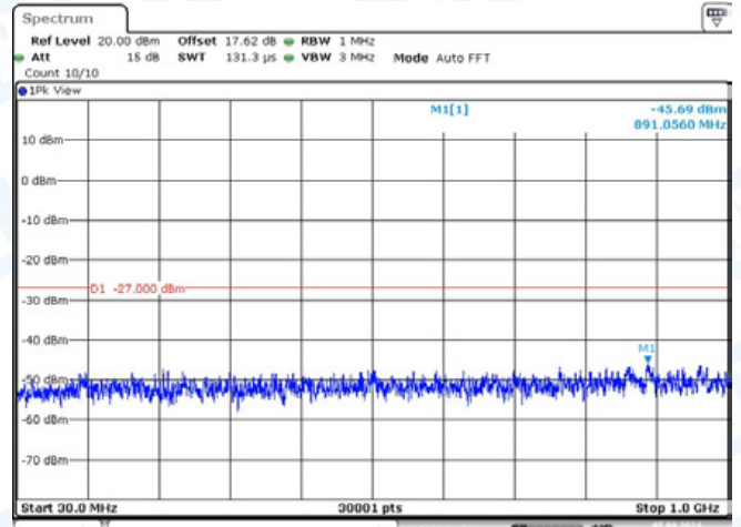
11AC40-CDD-Ant1-5550-30~1000-PASS
