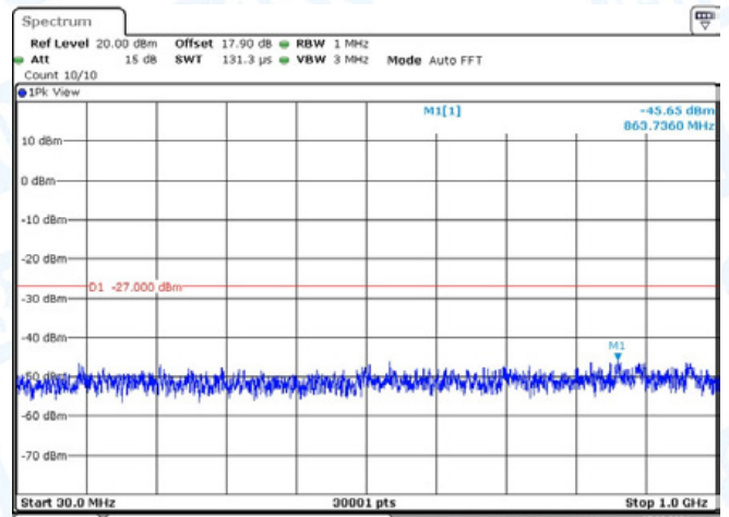
11AC40-CDD-Ant2-5550-30~1000-PASS
