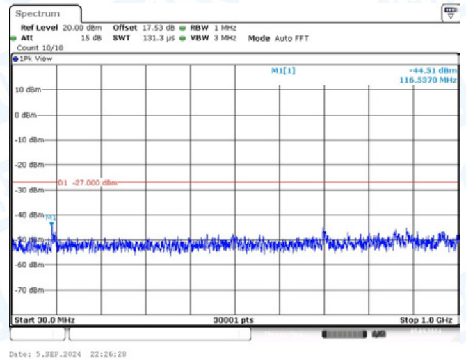
11AC80-CDD-Ant2-5290-30~1000-PASS
