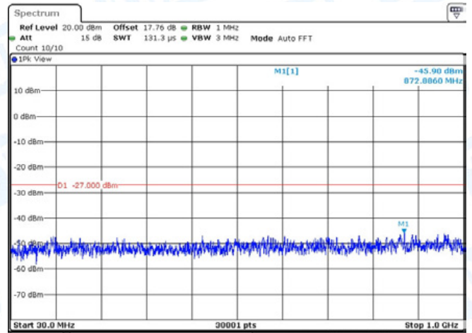
11AC40-CDD-Ant1-5795-30~1000-PASS
