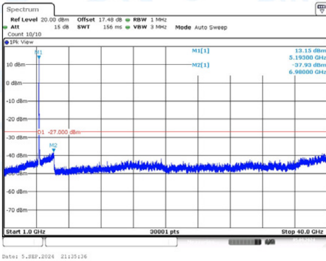
11AC40-CDD-Ant2-5190-1000~40000-PASS
