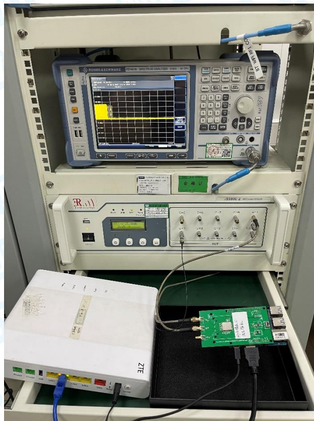
Photo of Setup for DFS Test
