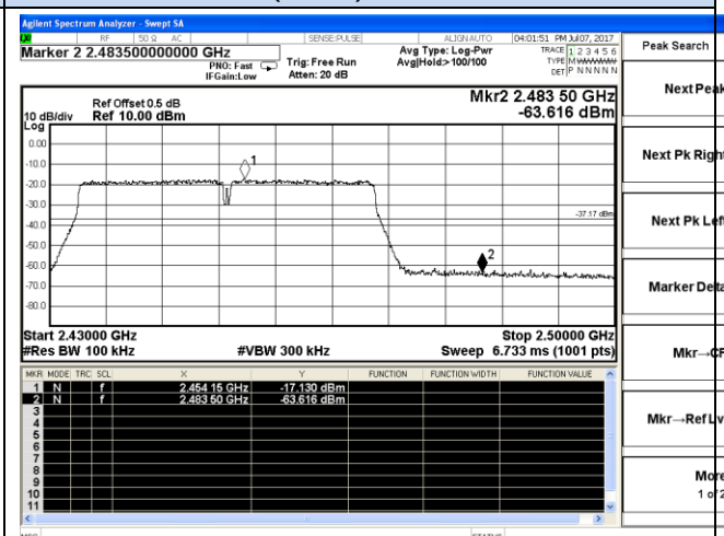
802.11n(HT40)-High channel
