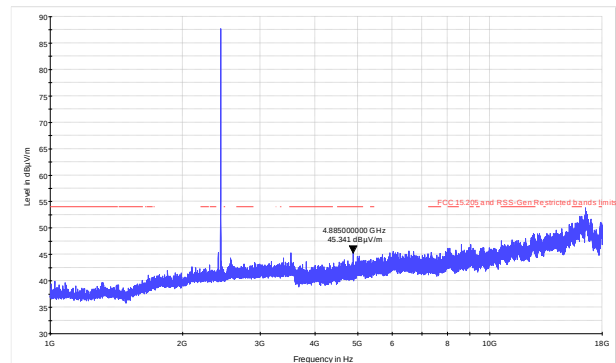
Figure 8.3-12: Radiated spurious emissions above 1 GHz, mid channel
