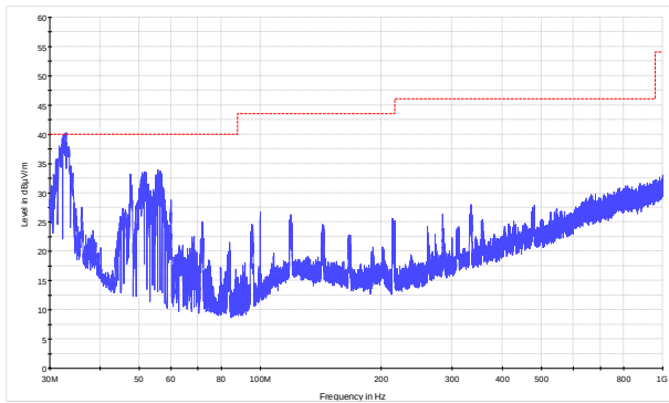
Figure 8.3-9: Radiated spurious emissions below 1 GHz, mid channel
