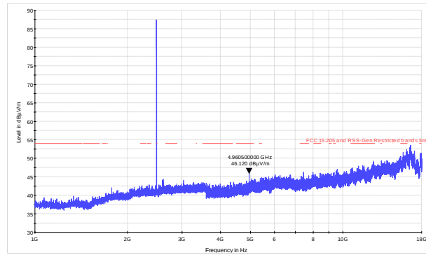
Figure 8.3-13: Radiated spurious emissions above 1 GHz, high channel
