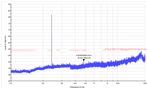
Figure 8.3-11: Radiated spurious emissions above 1 GHz, low channel
