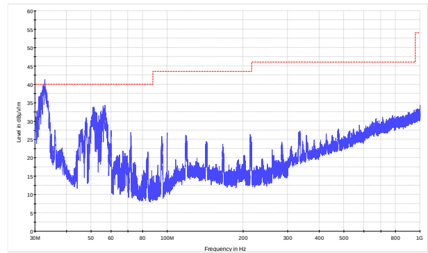
Figure 8.3-10: Radiated spurious emissions below 1 GHz, high channel
