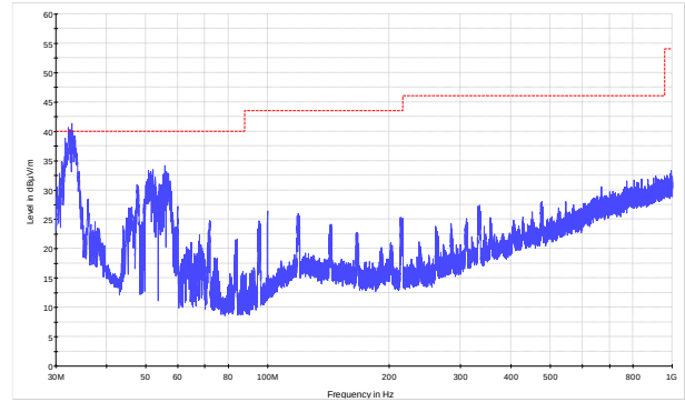
Figure 8.3-8: Radiated spurious emissions below 1 GHz, low channel
