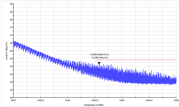
Figure 8.3-7: Radiated spurious emissions at the upper restricted band edge, low channel
