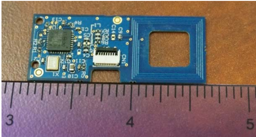
RFID Reader Board Top Side
