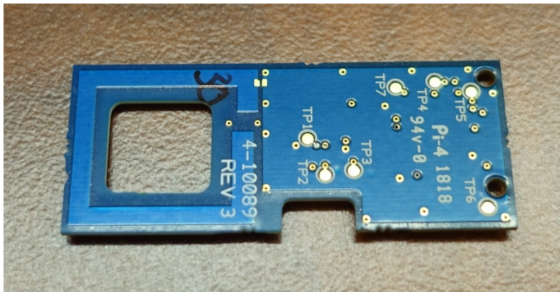
RFID Reader Board Solder Side
