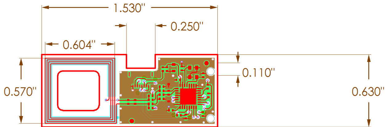
RFID Reader Board Layout
