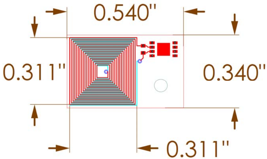
RFID Tag Board Layout
