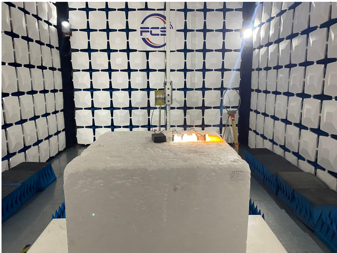
RE (Above1GHz)
