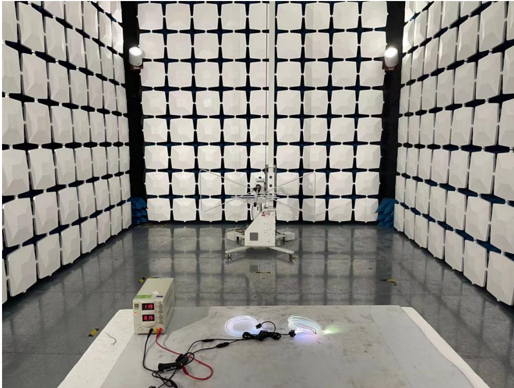
Blow 1GHz for radiated emission test setup
