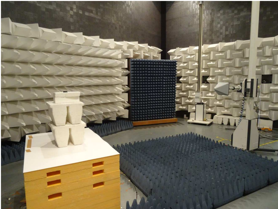
Radiated emission 1GHz - 10 GHz
