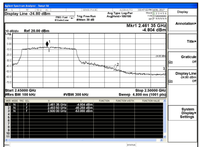
802.11n-HT20-High channel
