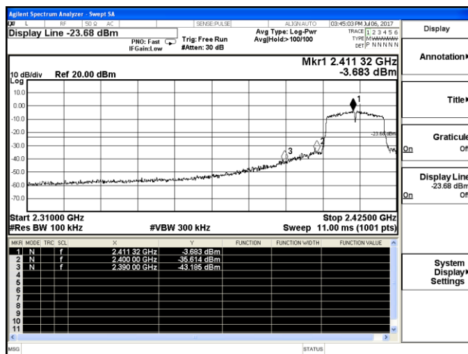
802.11n-HT20-Low channel
