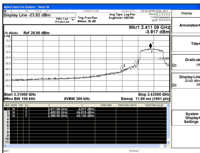
802.11g-Low channel
