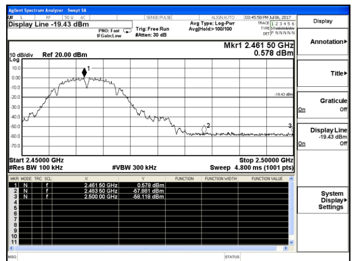
802.11b-High channel
