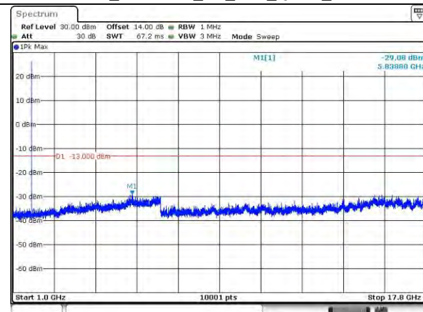
LTE Band 66_1745 MHz_5M_1RB_QPSK_Above 1GHz
