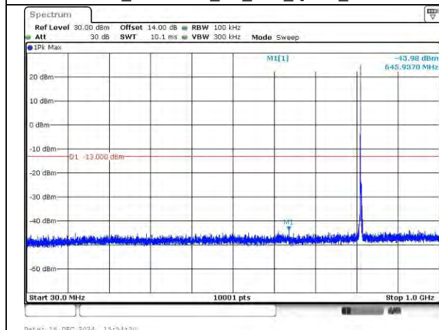
LTE Band 26_819 MHz_3M_1RB_QPSK_Below 1GHz
