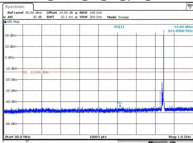
LTE Band 26_844 MHz_10M_1RB_QPSK_Below 1GHz
