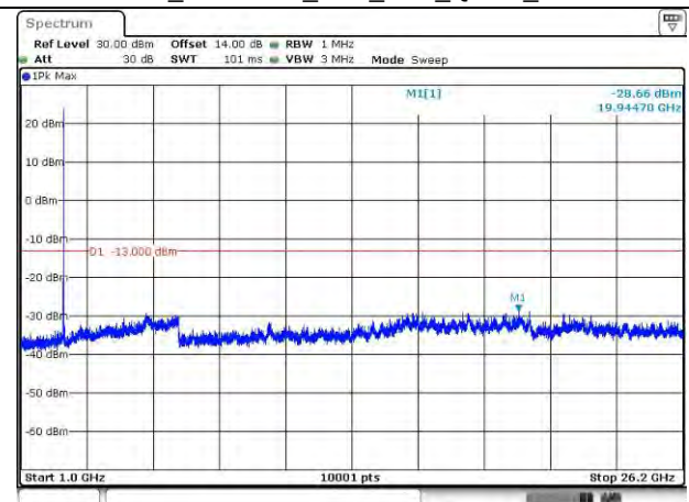
LTE Band 38_2615 MHz_10M_1RB_QPSK_Above 1GHz
