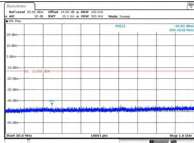
LTE Band 38_2572.5 MHz_5M_1RB_QPSK_Below 1GHz
