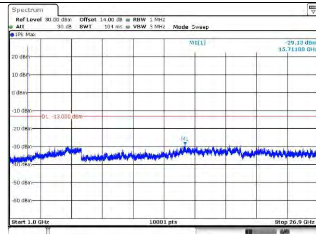
LTE Band 41_2498.5 MHz_5M_1RB_QPSK_Above 1GHz
