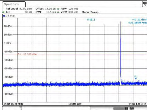
LTE Band 26_819 MHz_1.4M_1RB_QPSK_Below 1GHz
