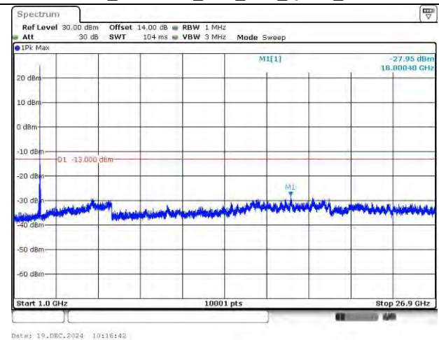
LTE Band 41_2682.5 MHz_15M_1RB_QPSK_Above 1GHz
