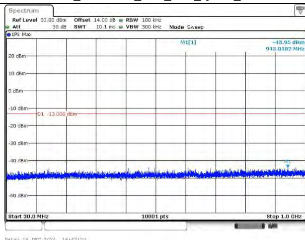
LTE Band 66_1770 MHz_20M_1RB_QPSK_Below 1GHz
