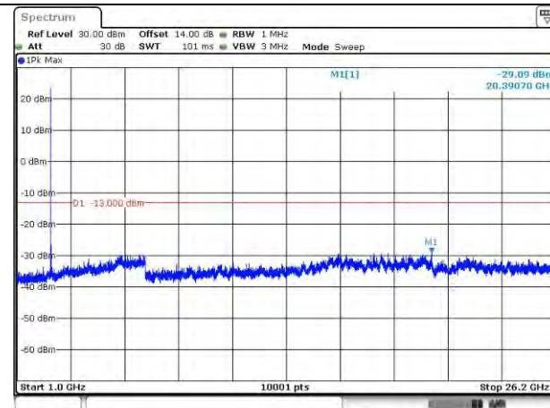
LTE Band 38_2572.5 MHz_5M_1RB_QPSK_Above 1GHz
