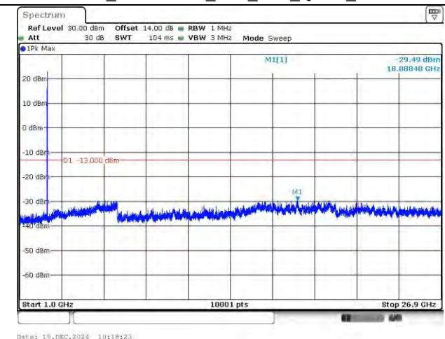
LTE Band 41_2682.5 MHz_15M_1RB_QPSK_Above 1GHz
