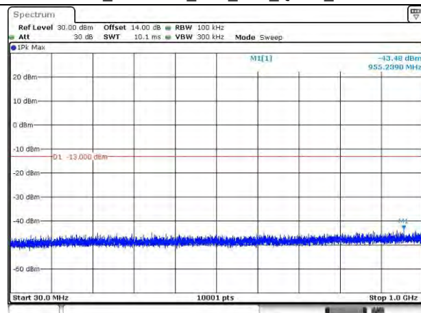
LTE Band 38_2615 MHz_10M_1RB_QPSK_Below 1GHz
