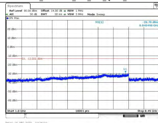
LTE Band 26_836.5 MHz_15M_1RB_QPSK_Above 1GHz
