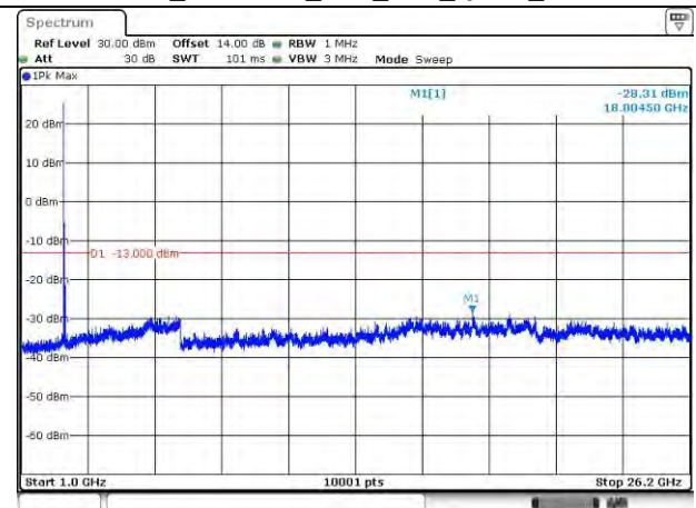
LTE Band 38_2595 MHz_10M_1RB_QPSK_Above 1GHz
