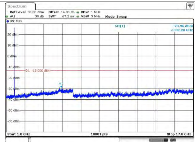
LTE Band 66_1745 MHz_15M_1RB_QPSK_Above 1GHz
