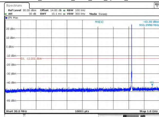
LTE Band 26_823.3 MHz_1.4M_1RB_QPSK_Below 1GHz
