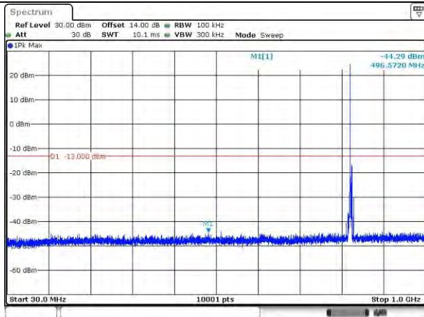
LTE Band 26_826.5 MHz_5M_1RB_QPSK_Below 1GHz
