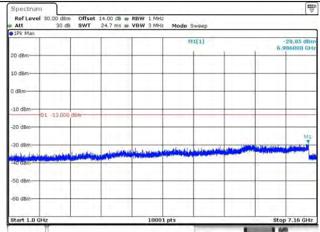
LTE Band 12_707.5 MHz_5M_1RB_QPSK_Above 1GHz
