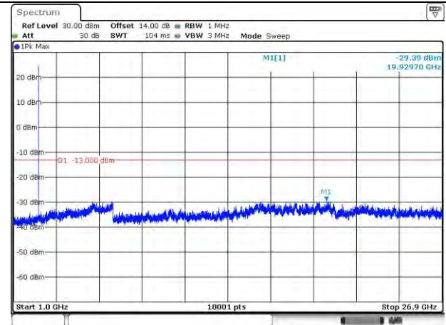
LTE Band 41_2501 MHz_10M_1RB_QPSK_Above 1GHz
