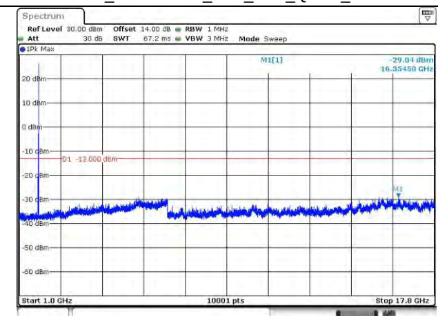
LTE Band 66_1772.5 MHz_15M_1RB_QPSK_Above 1GHz
