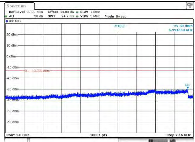
LTE Band 12_713.5 MHz_5M_1RB_QPSK_Above 1GHz
