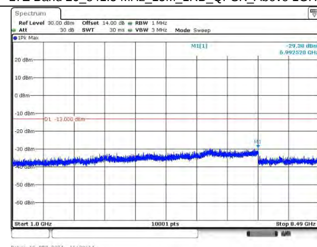
LTE Band 26_841.5 MHz_15M_1RB_QPSK_Above 1GHz
