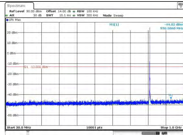
LTE Band 26_814.7 MHz_1.4M_1RB_QPSK_Below 1GHz
