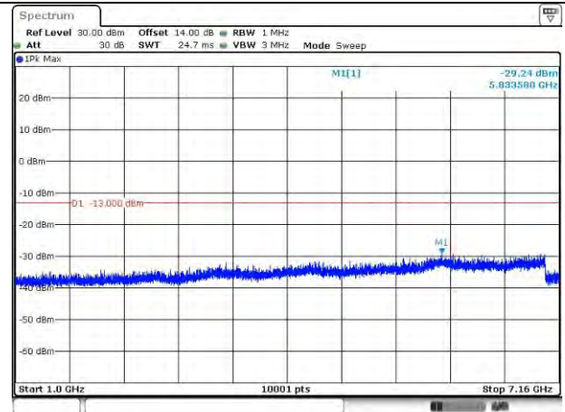
LTE Band 12_701.5 MHz_5M_1RB_QPSK_Above 1GHz
