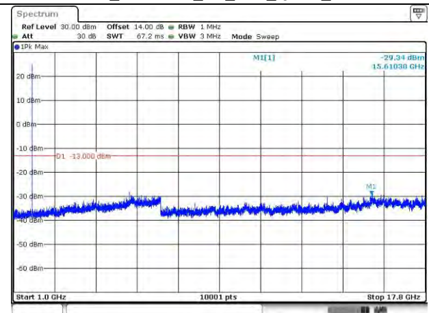
LTE Band 66_1745 MHz_3M_1RB_QPSK_Above 1GHz
