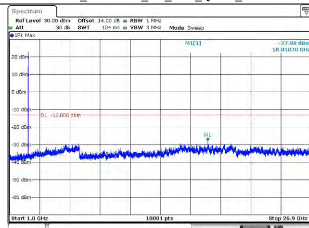
LTE Band 41_2593 MHz_5M_1RB_QPSK_Above 1GHz
