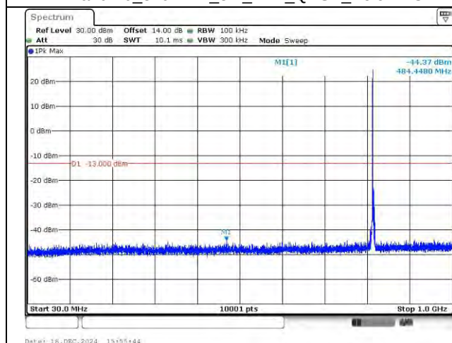
LTE Band 26_822.5 MHz_3M_1RB_QPSK_Below 1GHz
