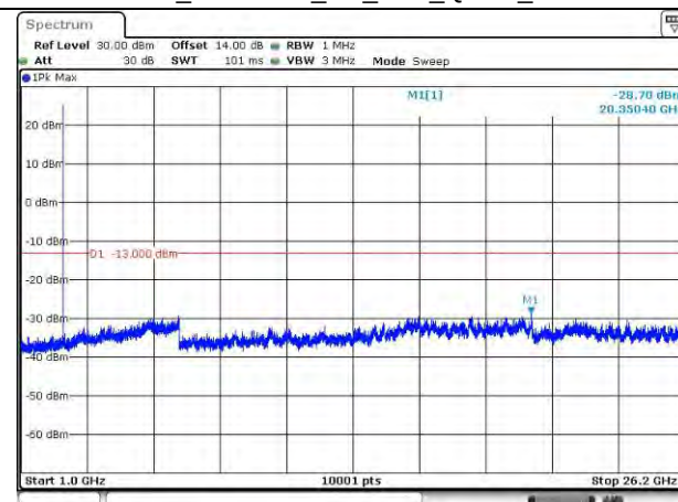
LTE Band 38_2595 MHz_5M_1RB_QPSK_Above 1GHz
