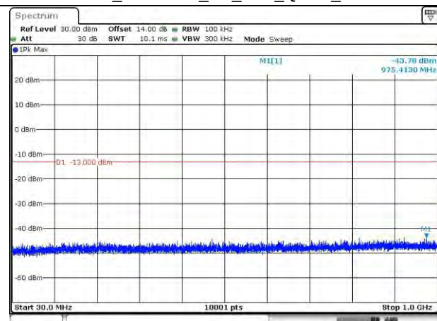
LTE Band 38_2595 MHz_5M_1RB_QPSK_Below 1GHz
