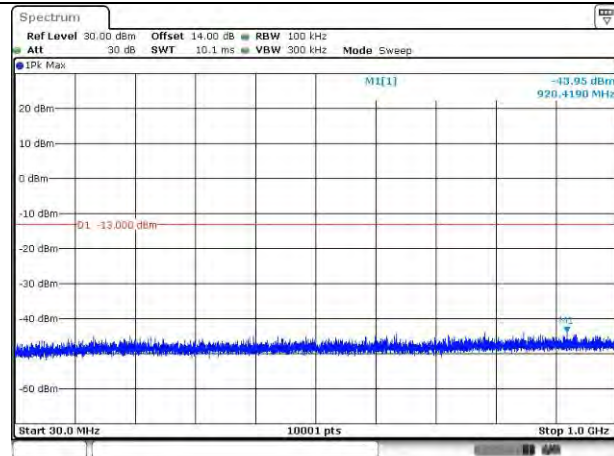
LTE Band 38_2580 MHz_20M_1RB_QPSK_Below 1GHz
