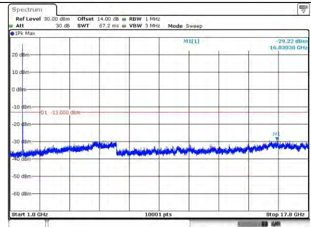
LTE Band 66_1711.5 MHz_3M_1RB_QPSK_Above 1GHz
