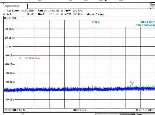
LTE Band 41_2685 MHz_10M_1RB_QPSK_Below 1GHz
