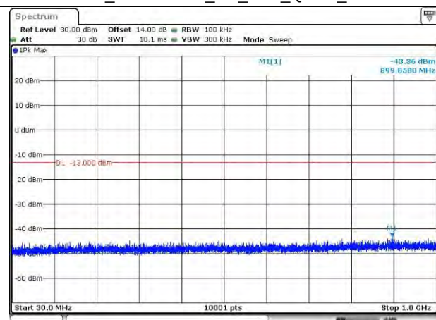
LTE Band 38_2617.5 MHz_5M_1RB_QPSK_Below 1GHz
