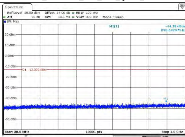
LTE Band 7_2565 MHz_10M_1RB_QPSK_Below 1GHz
