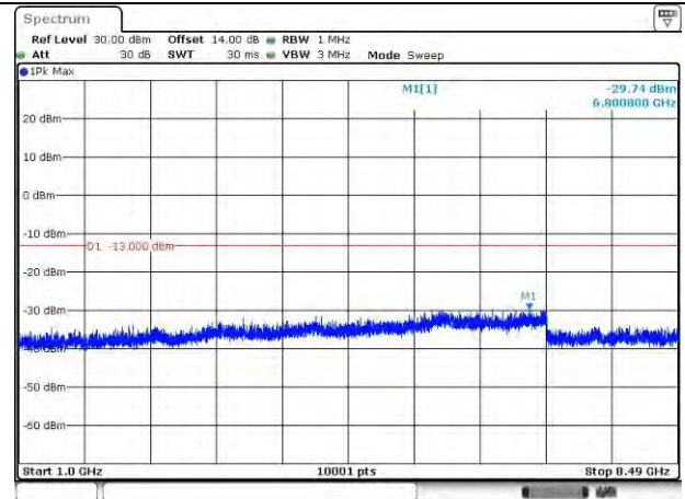
LTE Band 26_826.5 MHz_5M_1RB_QPSK_Above 1GHz
