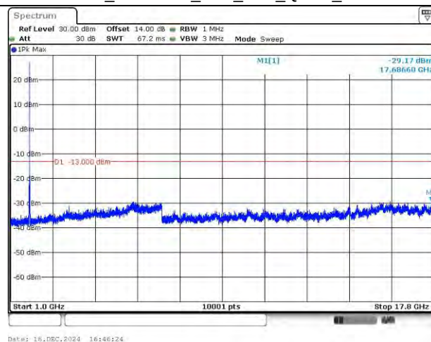
LTE Band 66_1770 MHz_20M_1RB_QPSK_Above 1GHz
