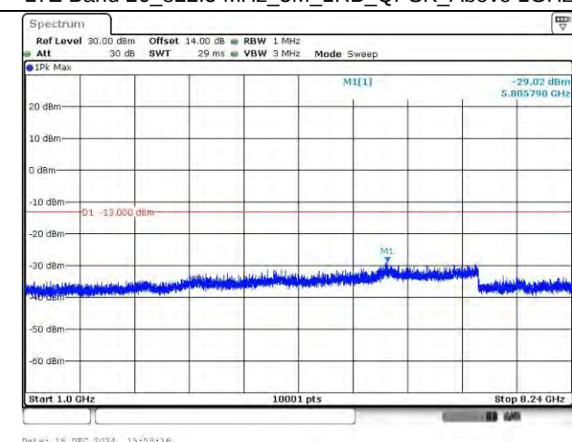
LTE Band 26_822.5 MHz_3M_1RB_QPSK_Above 1GHz
