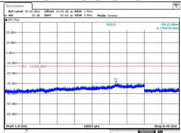
LTE Band 26_836.5 MHz_5M_1RB_QPSK_Above 1GHz
