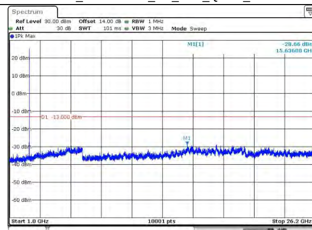
LTE Band 38_2617.5 MHz_5M_1RB_QPSK_Above 1GHz
