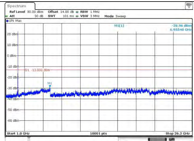
LTE Band 38_2610 MHz_20M_1RB_QPSK_Above 1GHz
