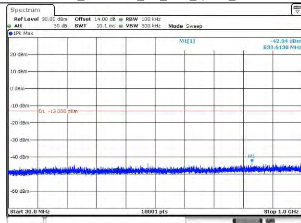
LTE Band 66_1745 MHz_3M_1RB_QPSK_Below 1GHz
