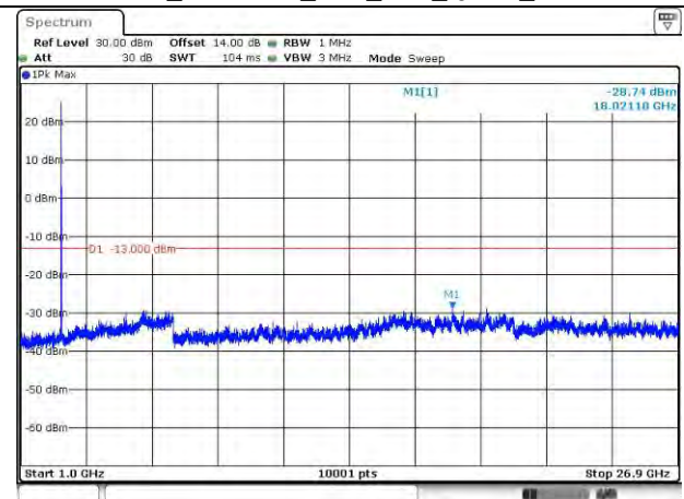
LTE Band 41_2593 MHz_10M_1RB_QPSK_Above 1GHz
