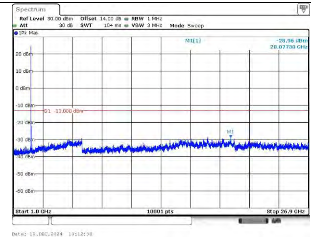
LTE Band 41_2593 MHz_15M_1RB_QPSK_Above 1GHz
