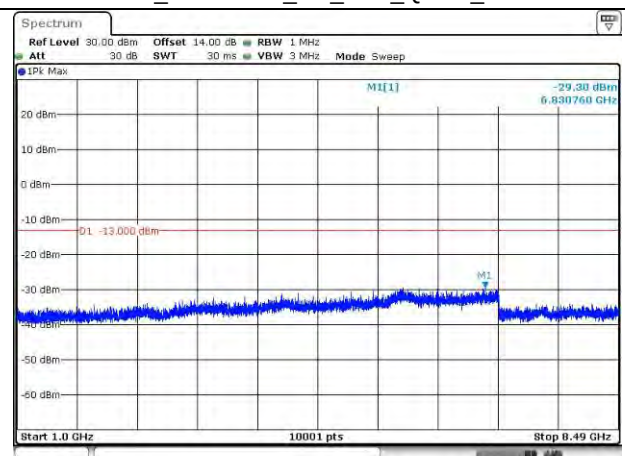
LTE Band 26_846.5 MHz_5M_1RB_QPSK_Above 1GHz
