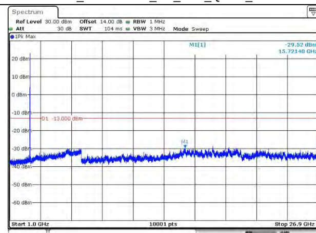
LTE Band 41_2687.5 MHz_5M_1RB_QPSK_Above 1GHz
