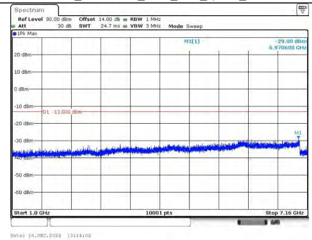
LTE Band 12_715.3 MHz_1.4M_1RB_QPSK_Above 1GHz
