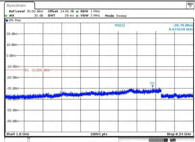
LTE Band 26_816.5 MHz_5M_1RB_QPSK_Above 1GHz
