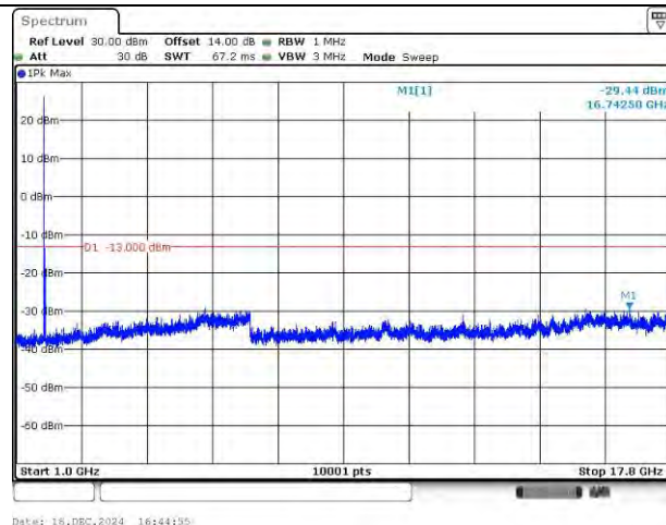
LTE Band 66_1745 MHz_20M_1RB_QPSK_Above 1GHz
