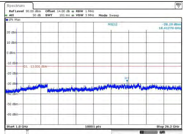
LTE Band 38_2575 MHz_10M_1RB_QPSK_Above 1GHz
