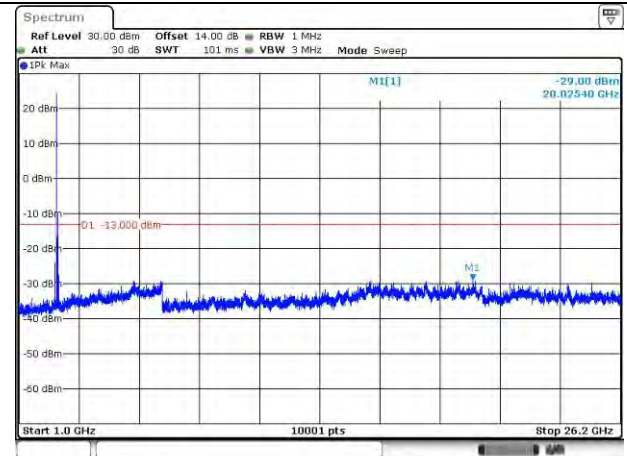
LTE Band 38_2580 MHz_20M_1RB_QPSK_Above 1GHz
