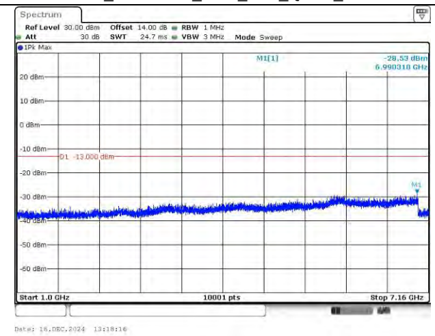
LTE Band 12_715.3 MHz_1.4M_1RB_QPSK_Above 1GHz
