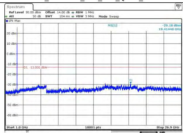
LTE Band 41_2685 MHz_10M_1RB_QPSK_Above 1GHz
