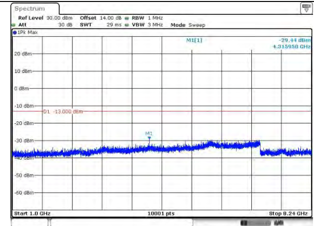
LTE Band 26_819 MHz_1.4M_1RB_QPSK_Above 1GHz
