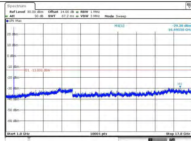
LTE Band 66_1712.5 MHz_5M_1RB_QPSK_Above 1GHz
