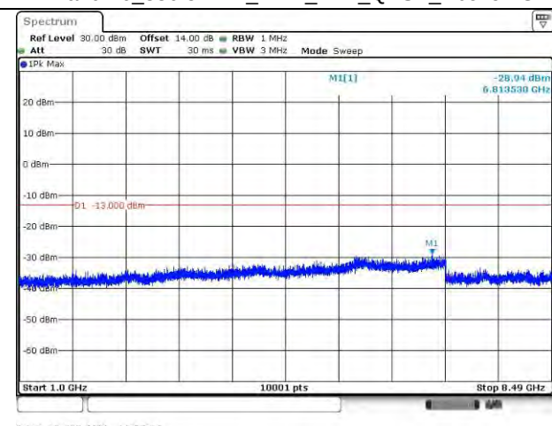
LTE Band 26_848.3 MHz_1.4M_1RB_QPSK_Above 1GHz
