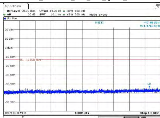
LTE Band 41_2680 MHz_20M_1RB_QPSK_Below 1GHz
