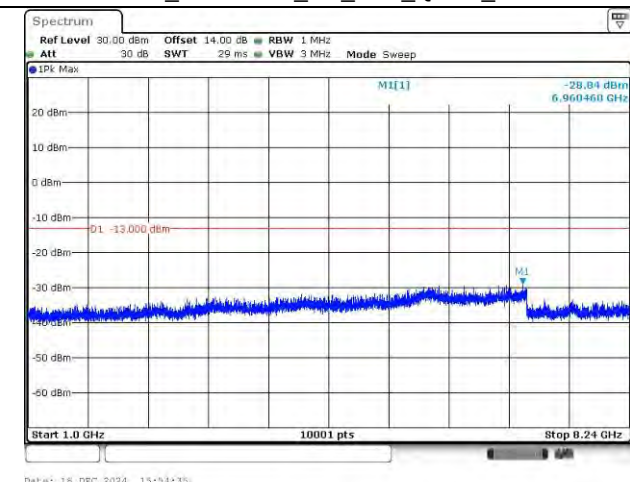
LTE Band 26_819 MHz_3M_1RB_QPSK_Above 1GHz
