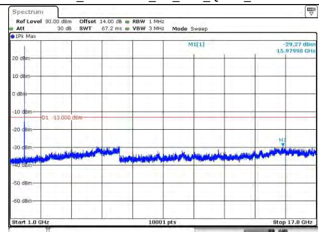
LTE Band 66_1778.5 MHz_3M_1RB_QPSK_Above 1GHz
