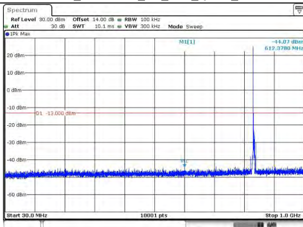
LTE Band 26_836.5 MHz_5M_1RB_QPSK_Below 1GHz
