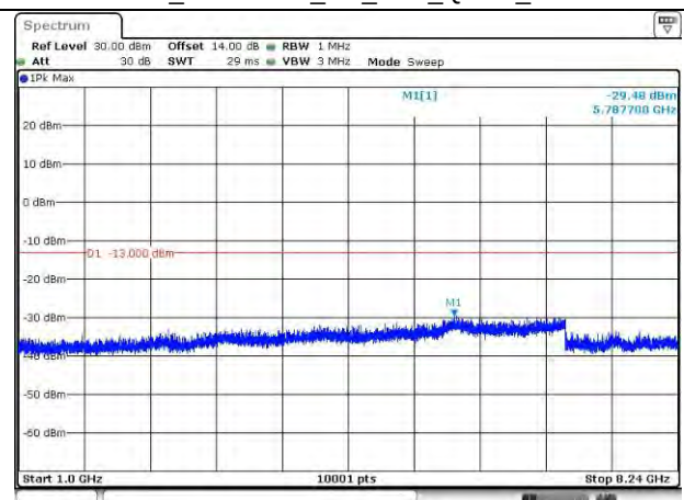
LTE Band 26_821.5 MHz_5M_1RB_QPSK_Above 1GHz
