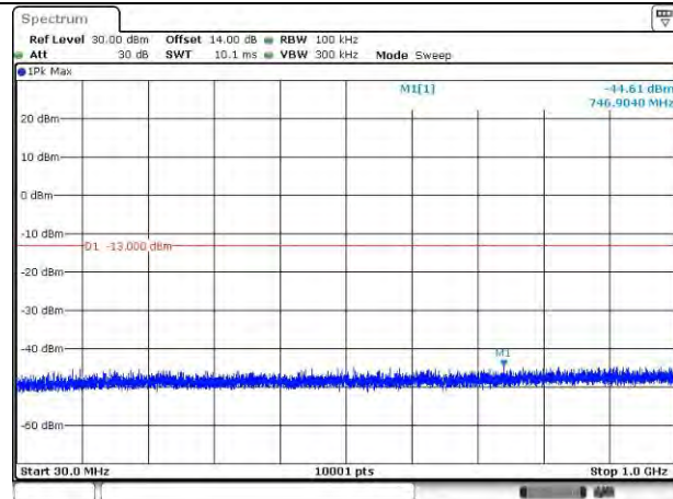
LTE Band 41_2501 MHz_10M_1RB_QPSK_Below 1GHz
