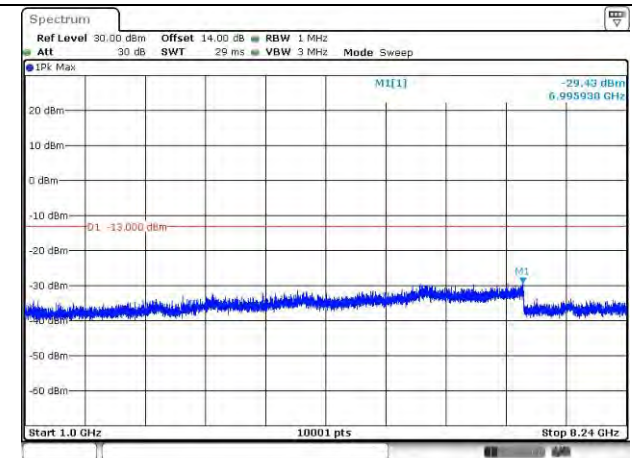
LTE Band 26_814.7 MHz_1.4M_1RB_QPSK_Above 1GHz
