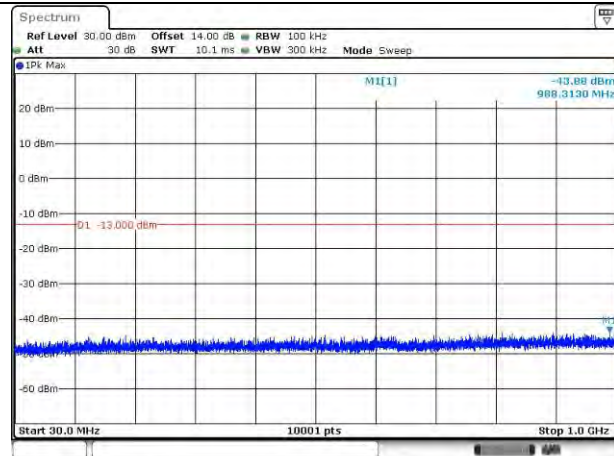
LTE Band 38_2595 MHz_20M_1RB_QPSK_Below 1GHz
