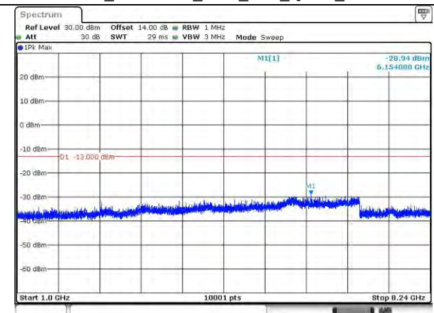
LTE Band 26_823.3 MHz_1.4M_1RB_QPSK_Above 1GHz
