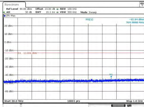
LTE Band 41_2506 MHz_20M_1RB_QPSK_Below 1GHz
