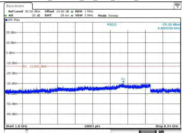
LTE Band 26_819 MHz_5M_1RB_QPSK_Above 1GHz
