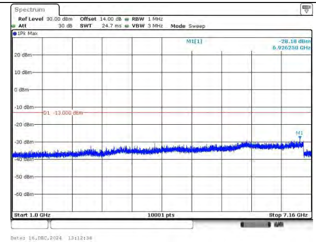
LTE Band 12_707.5 MHz_1.4M_1RB_QPSK_Above 1GHz
