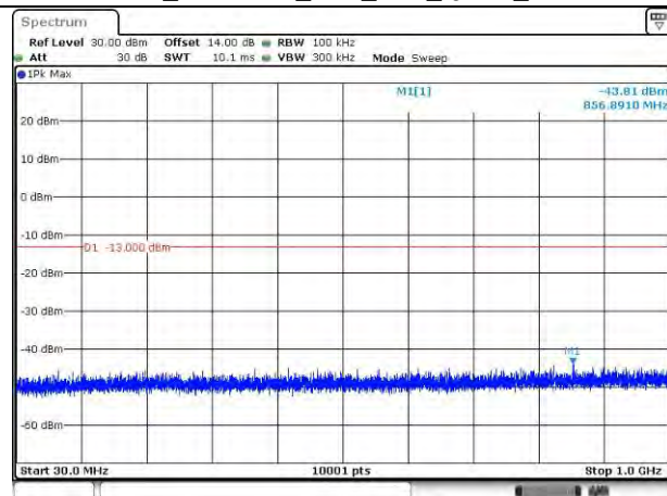
LTE Band 41_2593 MHz_10M_1RB_QPSK_Below 1GHz
