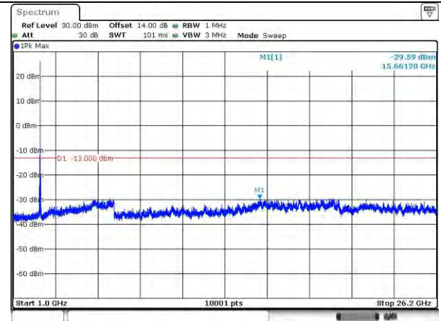
LTE Band 38_2595 MHz_20M_1RB_QPSK_Above 1GHz
