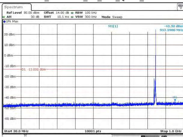
LTE Band 26_846.5 MHz_5M_1RB_QPSK_Below 1GHz
