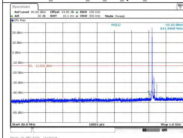
LTE Band 26_836.5 MHz_15M_1RB_QPSK_Below 1GHz
