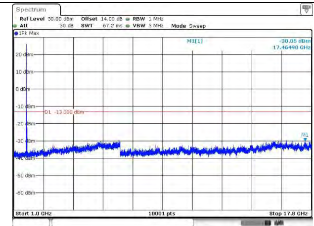
LTE Band 66_1717.5 MHz_15M_1RB_QPSK_Above 1GHz
