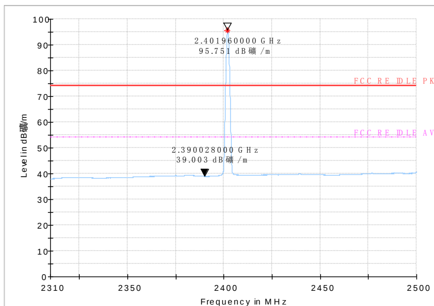
Fig.21 Bandedge:ch0
