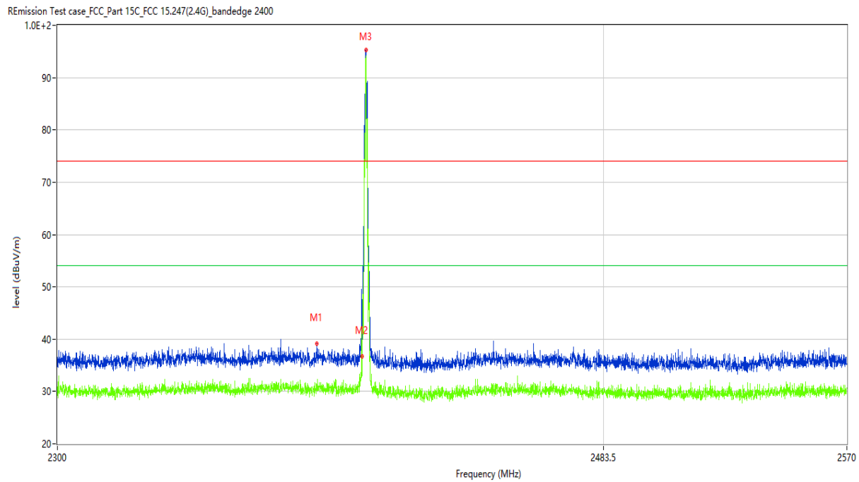
Figure 3: Band Edge (Restricted-band band-edge), 2402MHz, 8-DPSK
