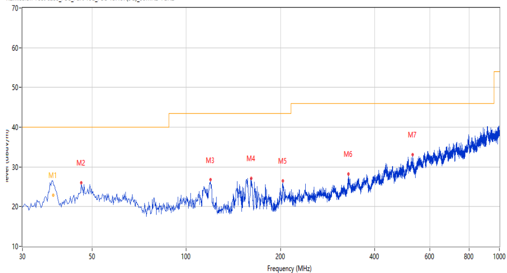
REmission Test case_FCC_Part 15E_FCC 15.407(5G)_30MHz-1GHz
