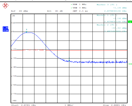
Frequency Band Edge: GFSK, Ch78, Hopping OFF
