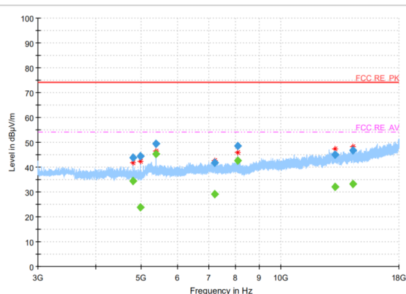
Radiated emission: GFSK, Ch0, 3GHz~18GHz
