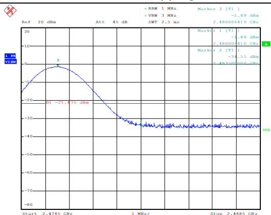
Frequency Band Edge: 8DPSK, Ch78, Hopping OFF
