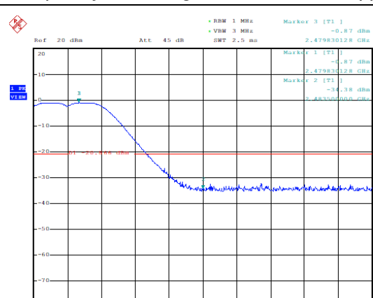
Frequency Band Edge: GFSK, Ch78, Hopping ON
