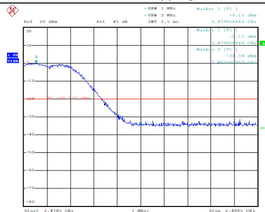
Frequency Band Edge: 8DPSK, Ch78, Hopping ON
