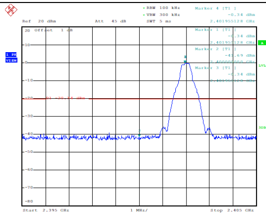
Frequency Band Edge: GFSK, Ch0, Hopping OFF
