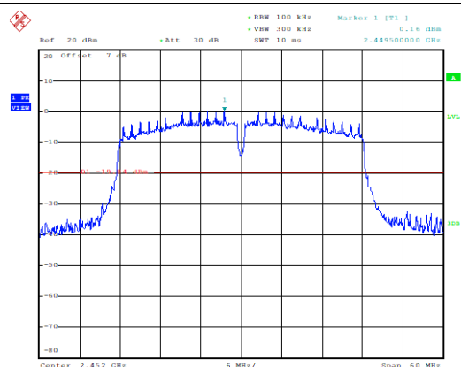
Conducted Spurious Emission (802.11n-40MHz, Ch9)
