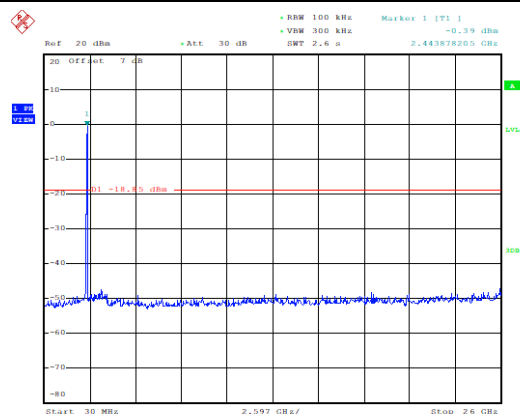
Conducted Spurious Emission (802.11n-40MHz, Ch6, 30MHz~26GHz)
