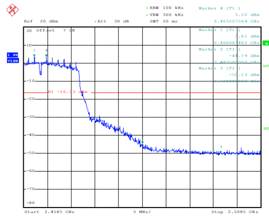
Band Edges (802.11g, Ch11)
