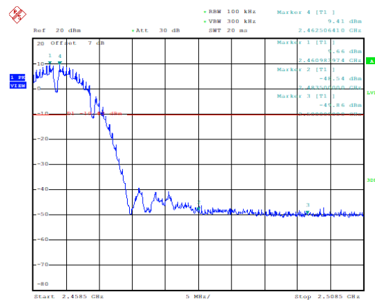
Band Edges (802.11b, Ch11)
