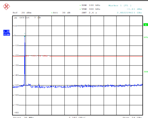
Conducted Spurious Emission (802.11n-40MHz, Ch3, 30MHz~26GHz)
