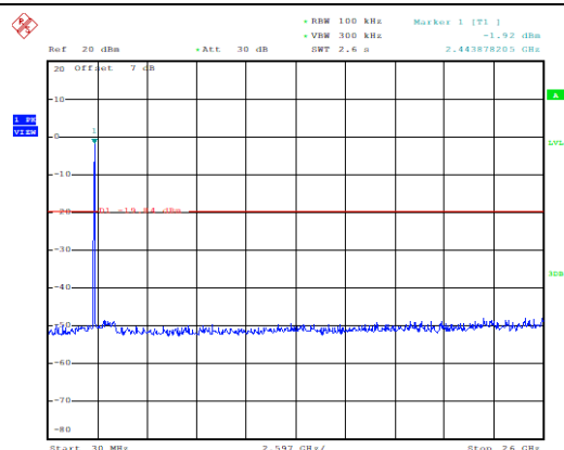
Conducted Spurious Emission (802.11n-40MHz, Ch9, 30MHz~26GHz)
