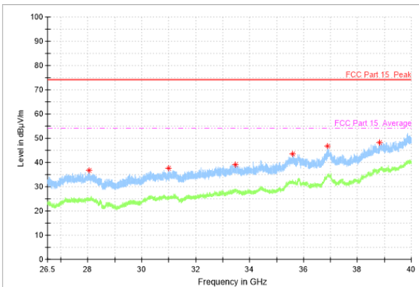
Radiated Spurious Emission (802.11ac-VHT80, ch155, 26.5GHz-40GHz)
