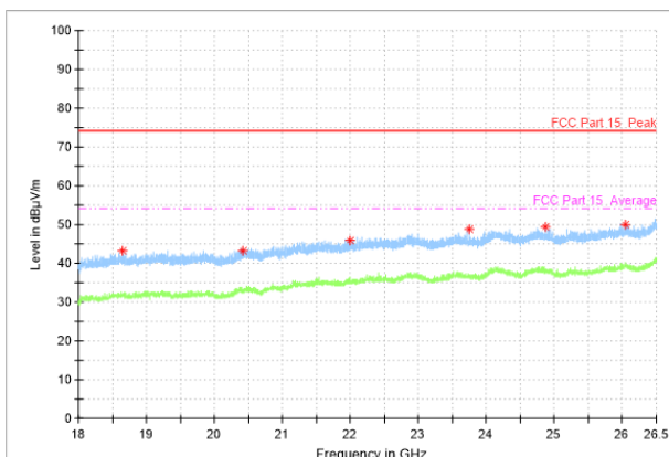
Radiated Spurious Emission (802.11ac-VHT80, ch155, 18GHz-26.5GHz)
