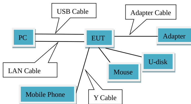
<Figure 2> Mode 10
