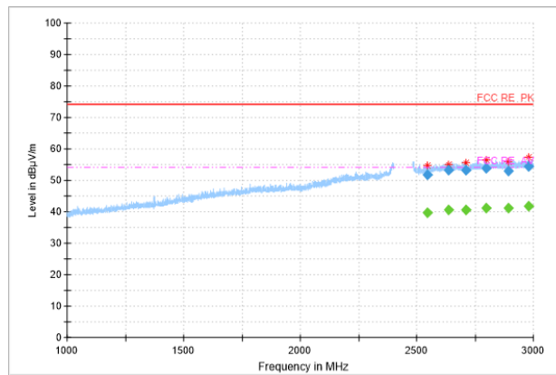
Bandedge: Ch39
