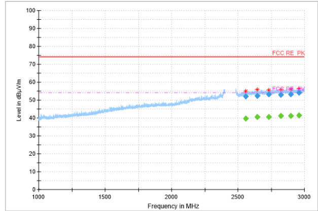
Bandedge:Ch39
