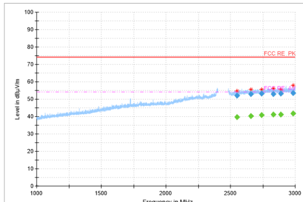
Bandedge:Ch39
