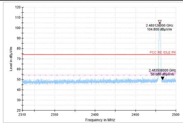
Bandedge:Ch39
