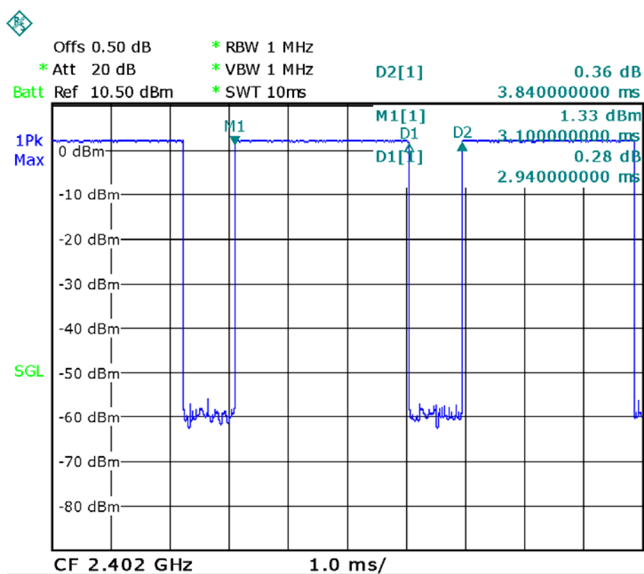
GFSK Low Channel
