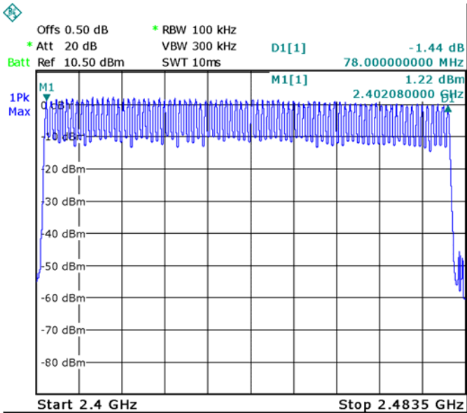
Modulation: GFSK
