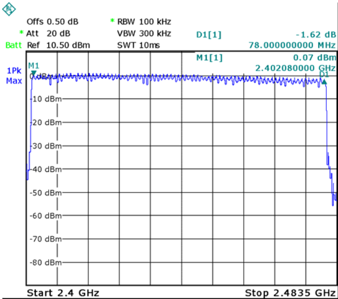
Modulation: 8DPSK
