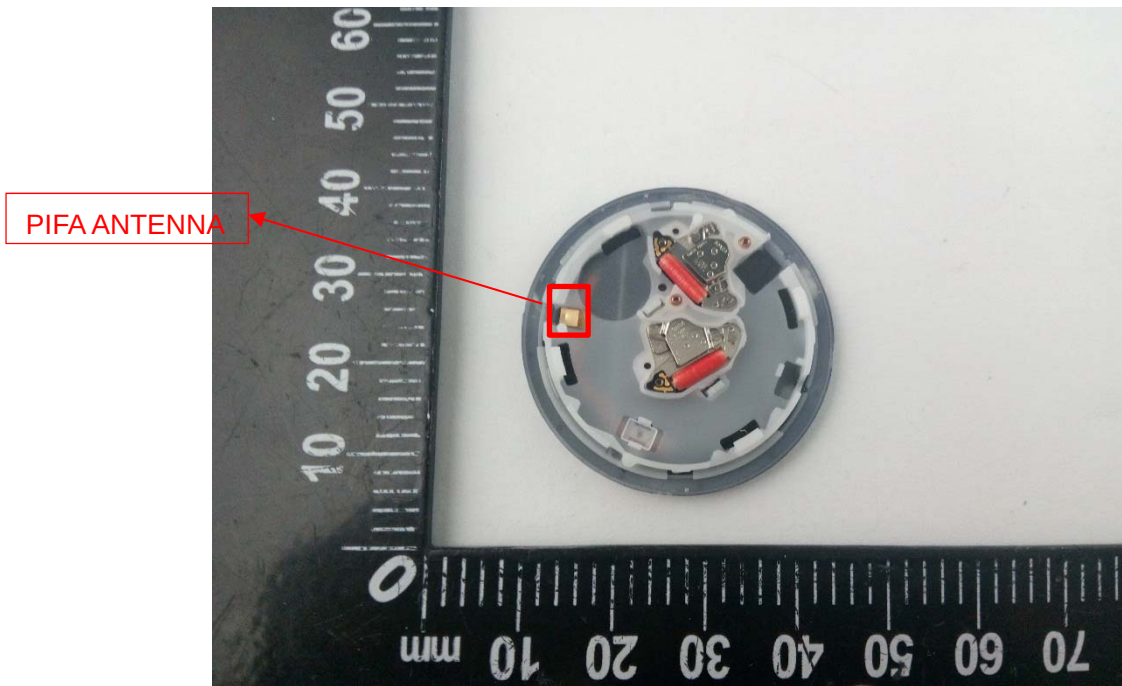
EUT UNCOVER VIEW 3(HCWA1M)
