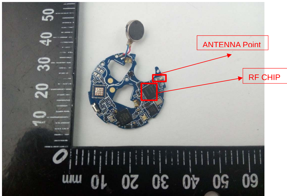
MAIN BOARD TOP VIEW 2(HCWA1M)
