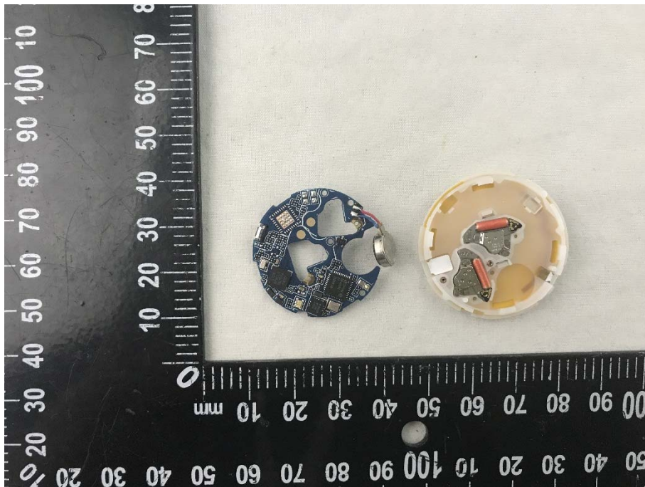
EUT UNCOVER VIEW 2(HCWA1F)
