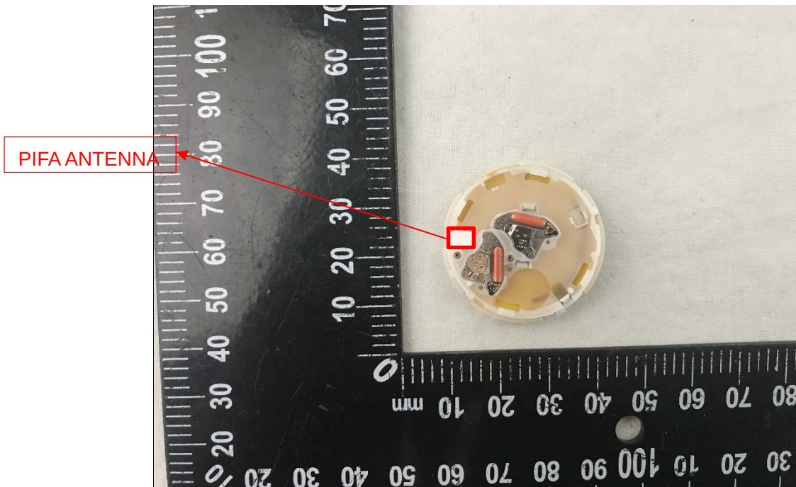
EUT UNCOVER VIEW 3(HCWA1F)
