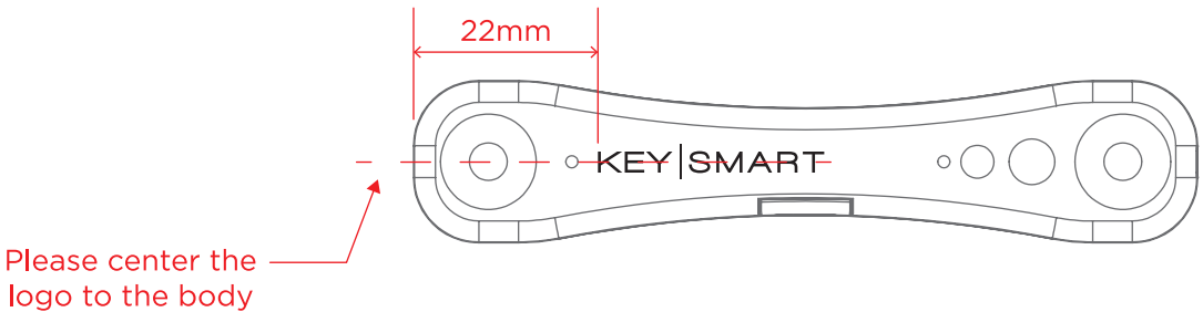
FRONT PLATE (OUTSIDE) Scale 1:1
