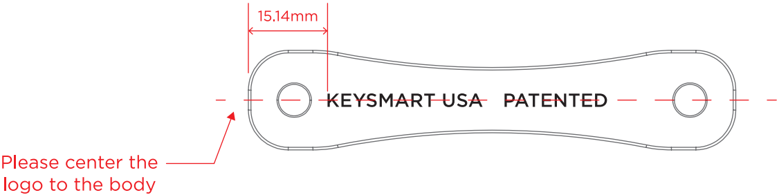
BACK PLATE (INSIDE) Scale 1:1
