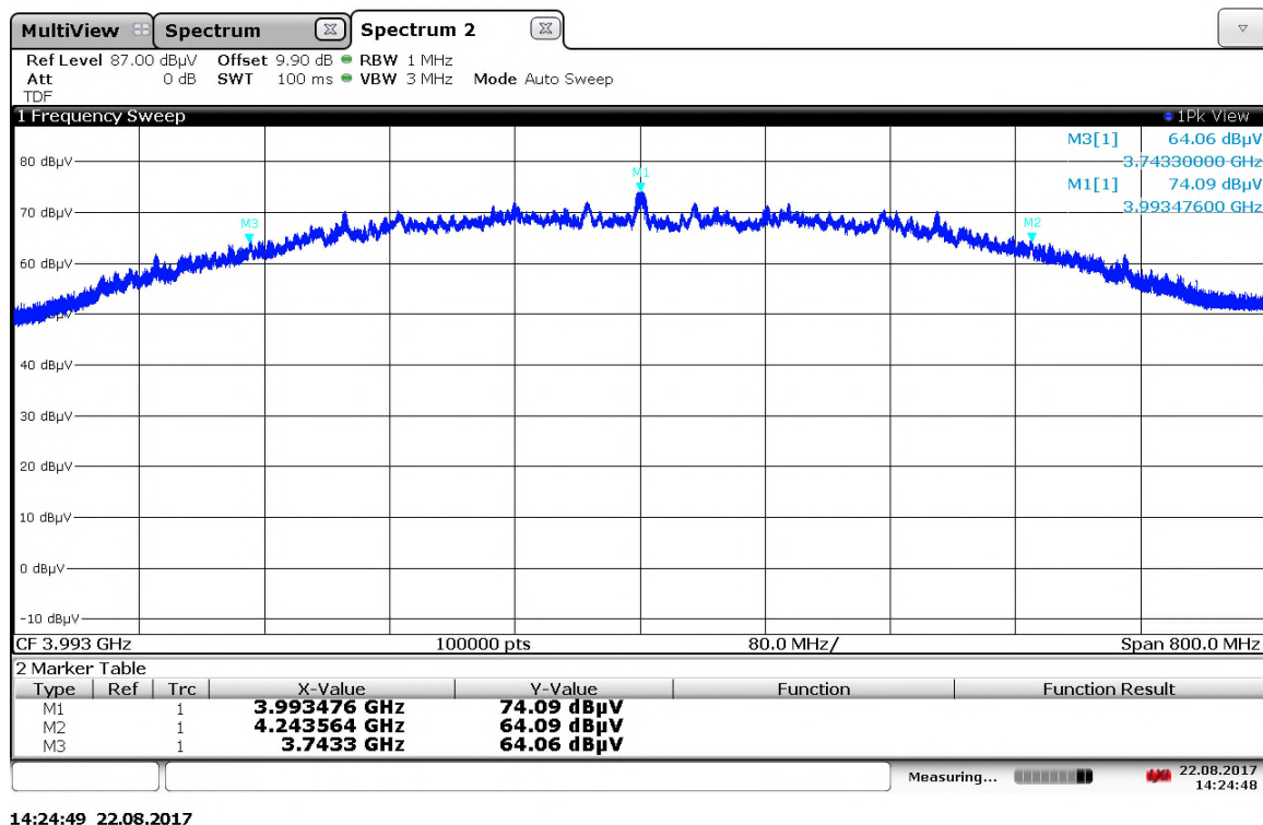
Figure 7.3.2-1: 10 dB Bandwidth
