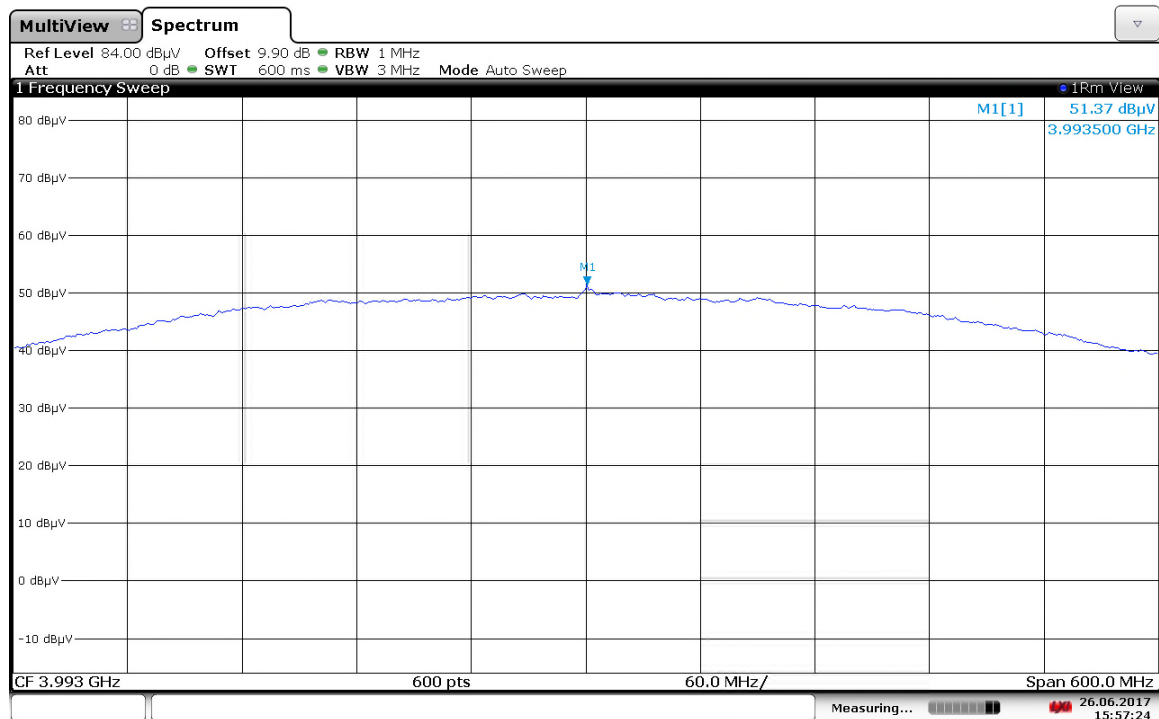
Figure 7.5.2-1: PSD Plot
