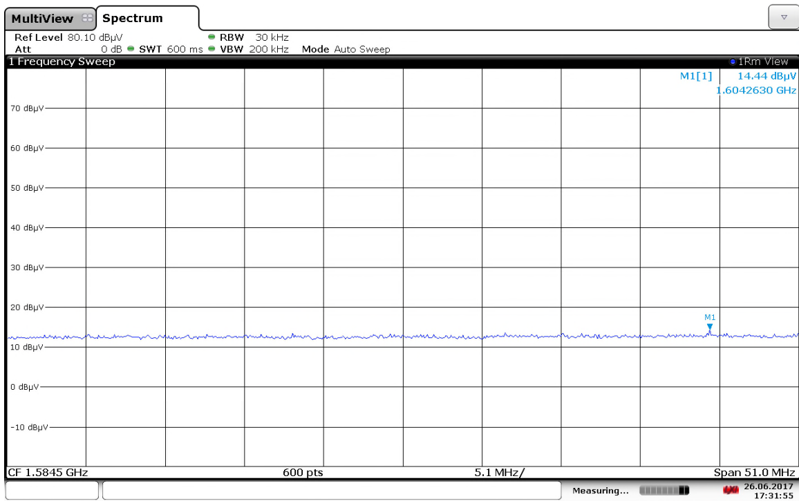
Figure 7.6.3.2-2: 1.559 GHz – 1.610 GHz
