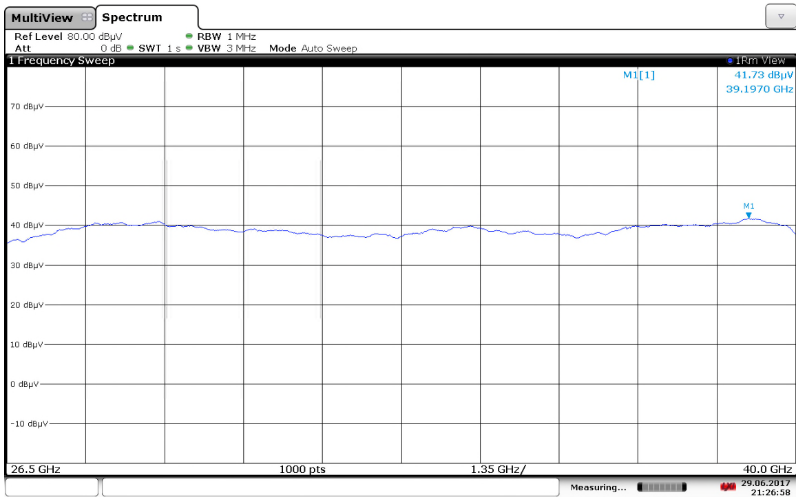
Figure 7.6.1.3-8: 26.5 GHz – 40 GHz
