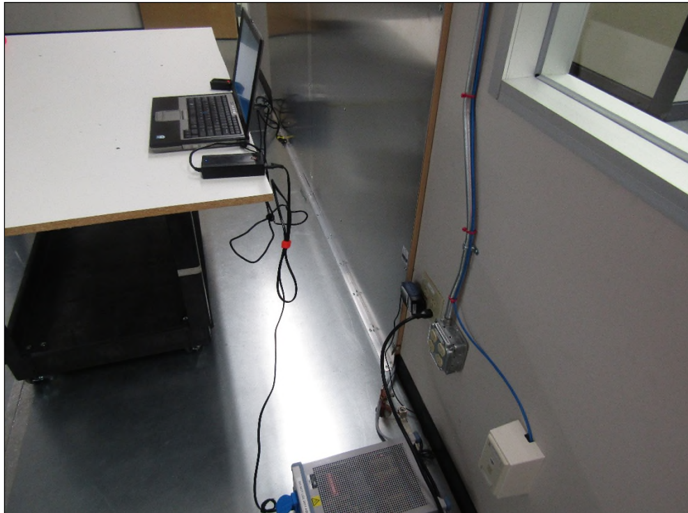
Figure 2: Power Line Conducted Emissions – Back View
