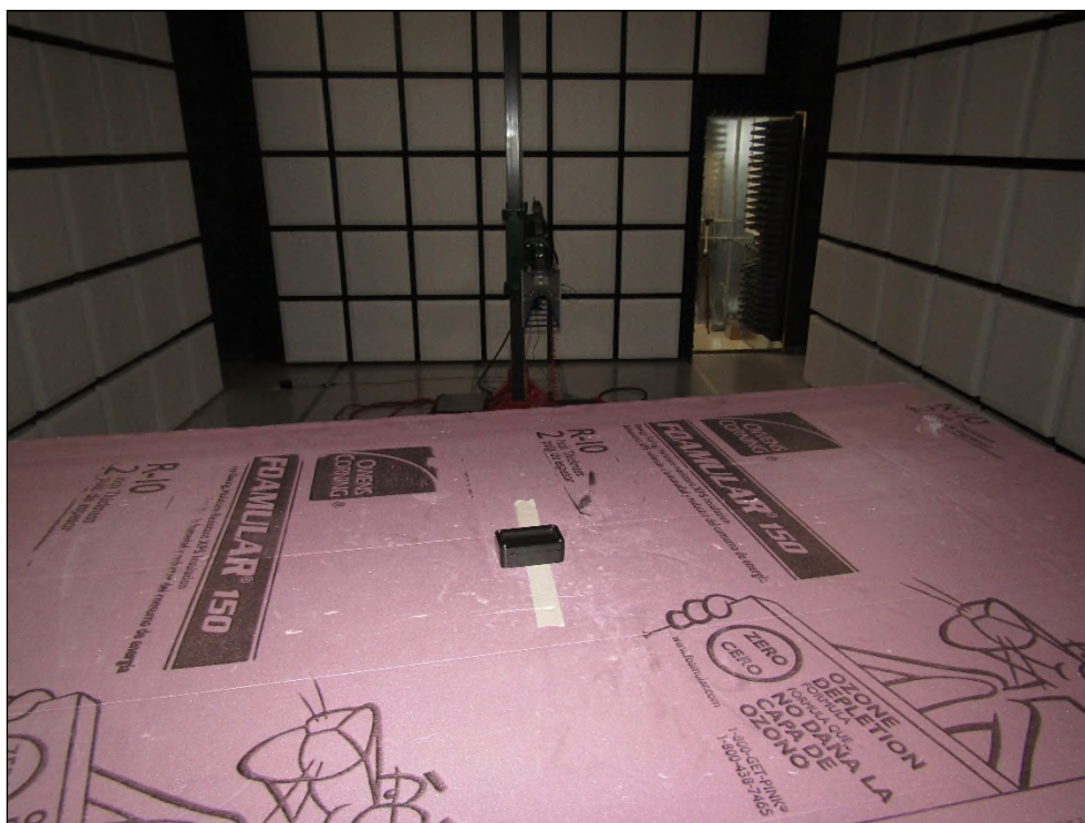
Figure 6: Radiated Emissions – Above 1GHz – Rear View
