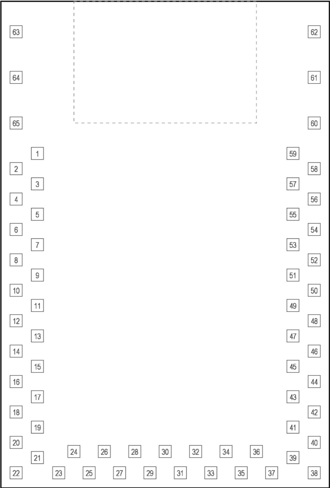
Figure 8: Pin Assignments
