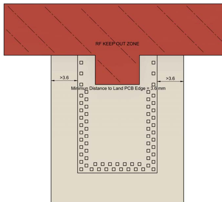
Figure 7: RF KEEP OUT ZONE (No Ground/Signals/Components)
