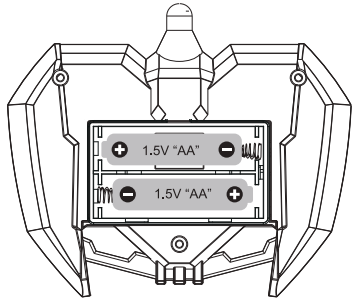
Back of Remote Controller
