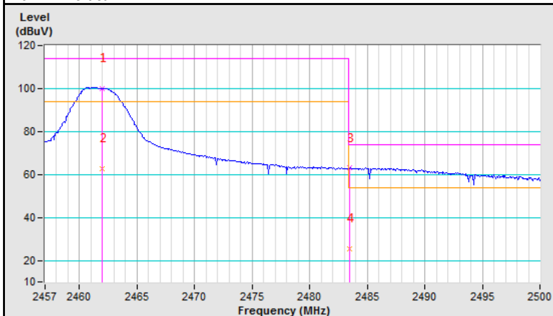
2462MHz Vertical
