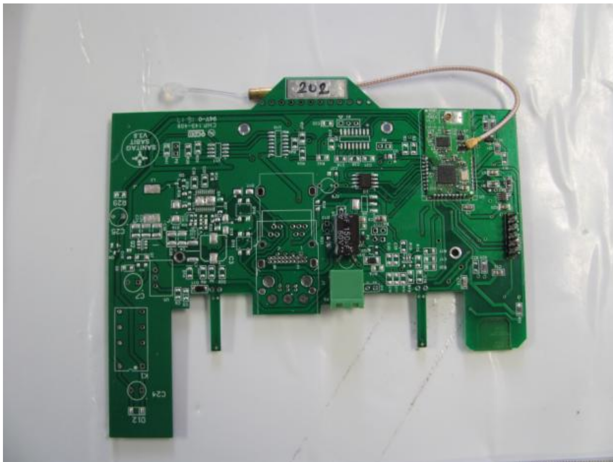
Figure 4. PCB Component View
