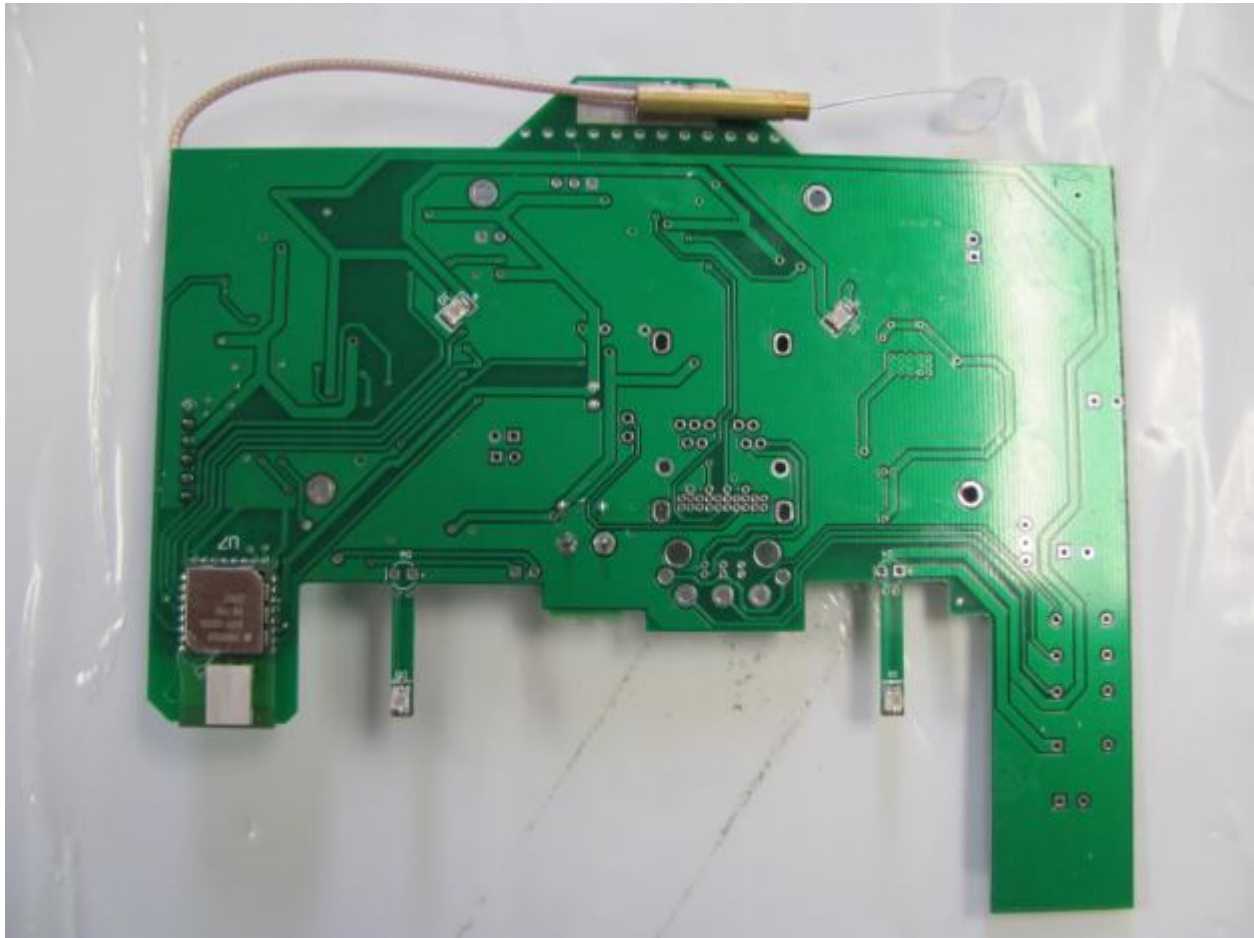
Figure 5. PCB Rear View
