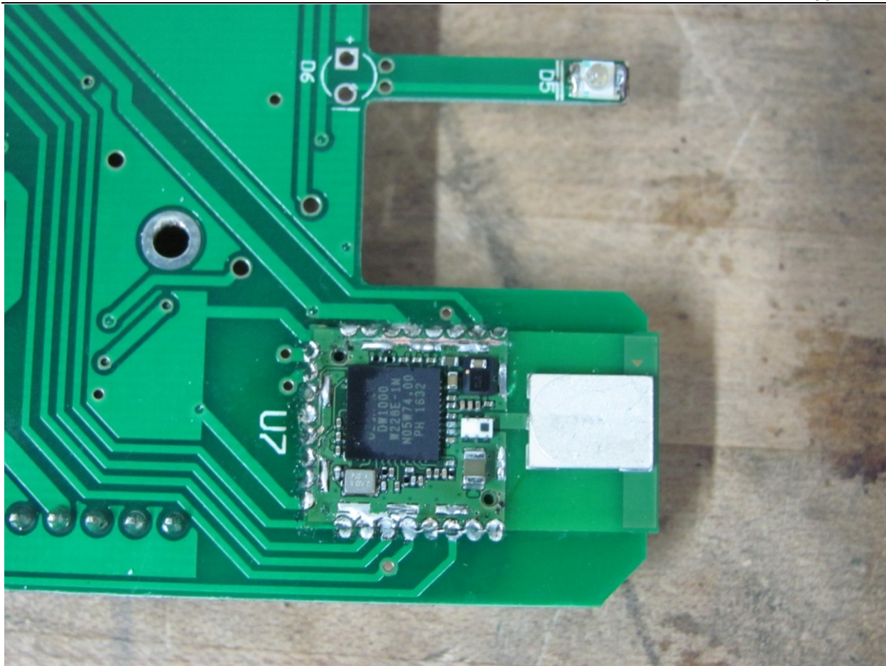
Figure 7. UWB Radio Module with Shield Removed
