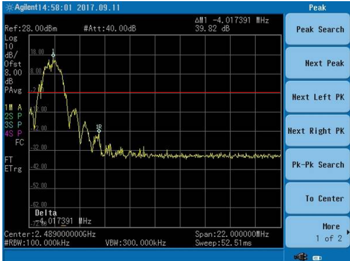
Figure 17. Band Edge Compliance, High Channel Delta – Average
