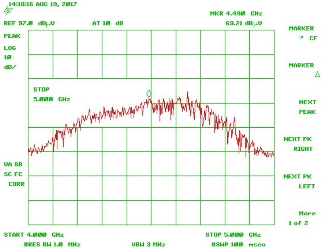
Figure 2. Fundamental Peak
