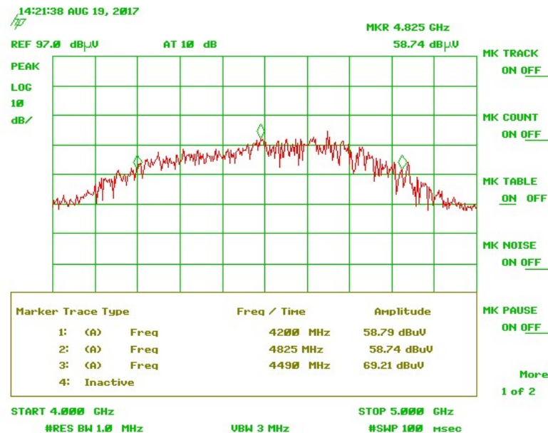
Figure 4. UWB 10 dB Bandwidth
