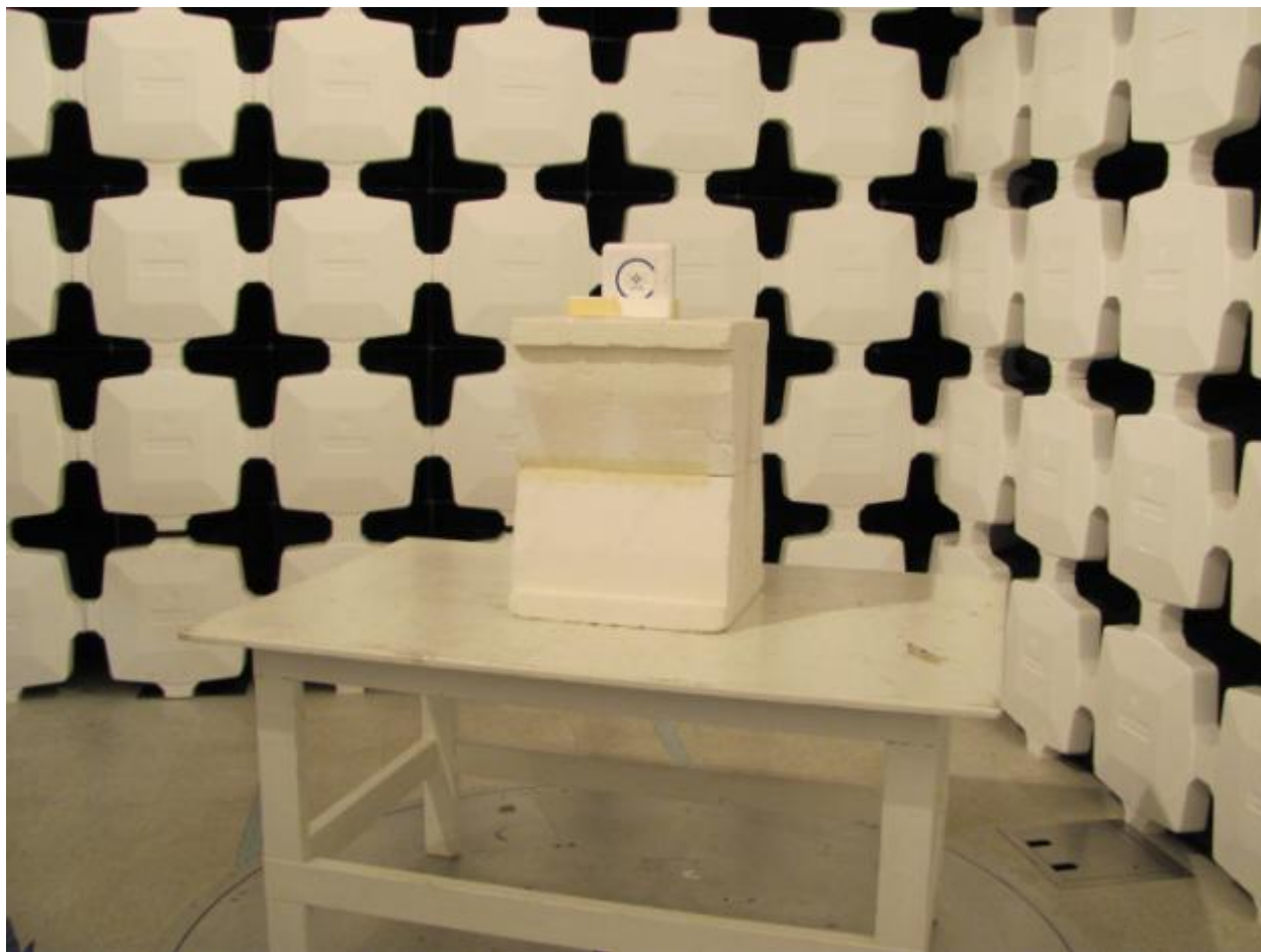
Figure 4. EUT on Raised Block for above 1 GHz Testing
