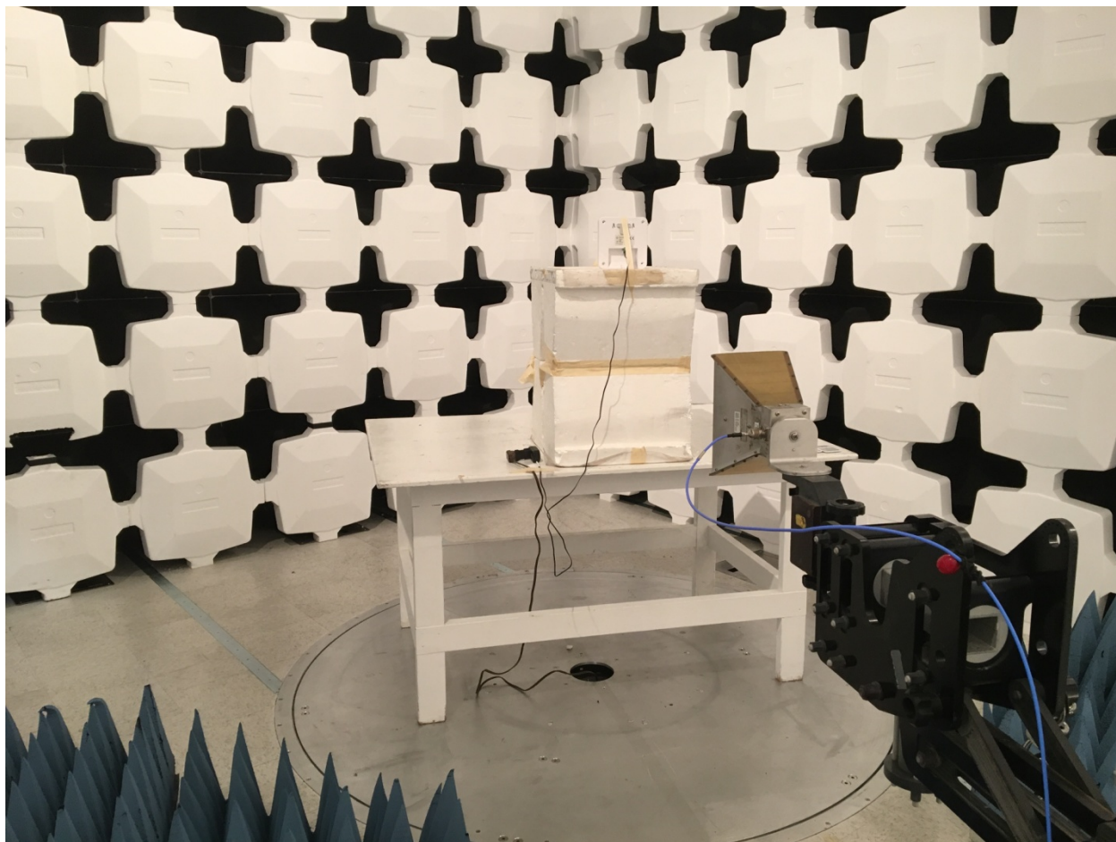
Figure 6. Radiated Emissions above 1 GHz at 1 Meter Distance
