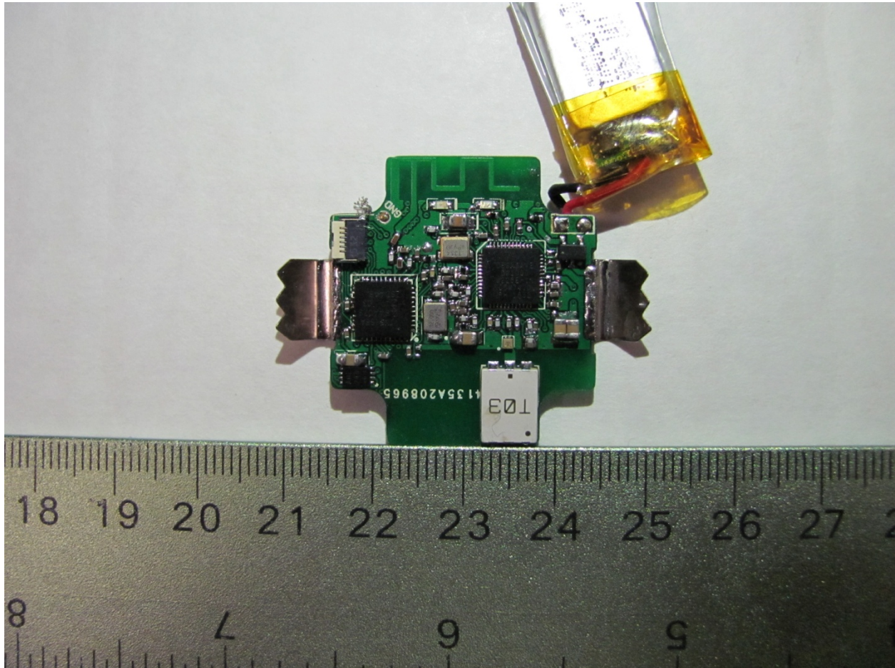
Figure 2. Front 2 Component Side
