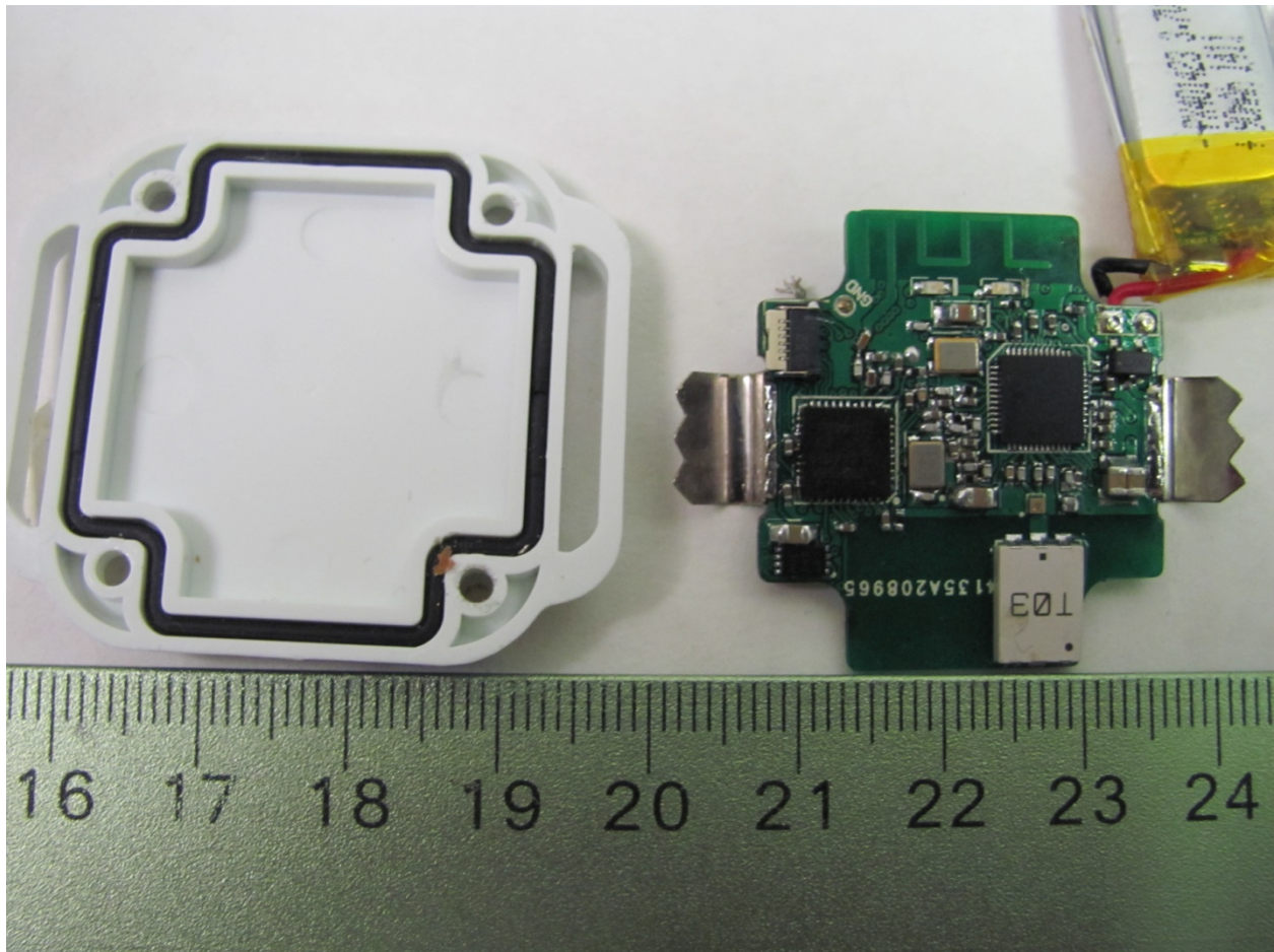
Figure 1. Front, Component Side
