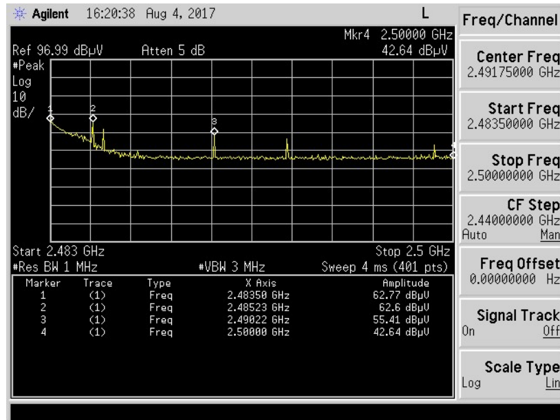
Figure 4. Radiated Restricted Band 2483.5 MHz to 2500 MHz, Peak
