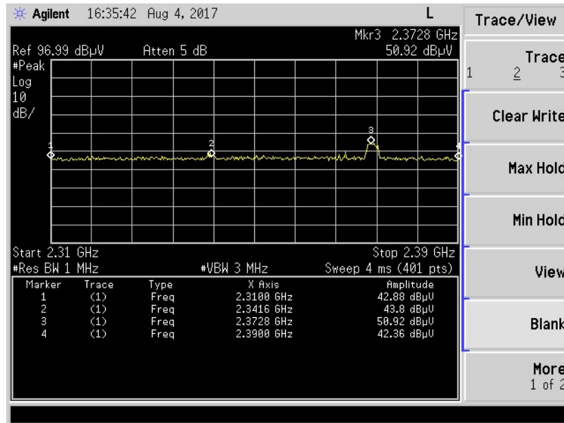
Figure 3. Radiated Restricted Band 2310 MHz to 2390 MHz, Peak
