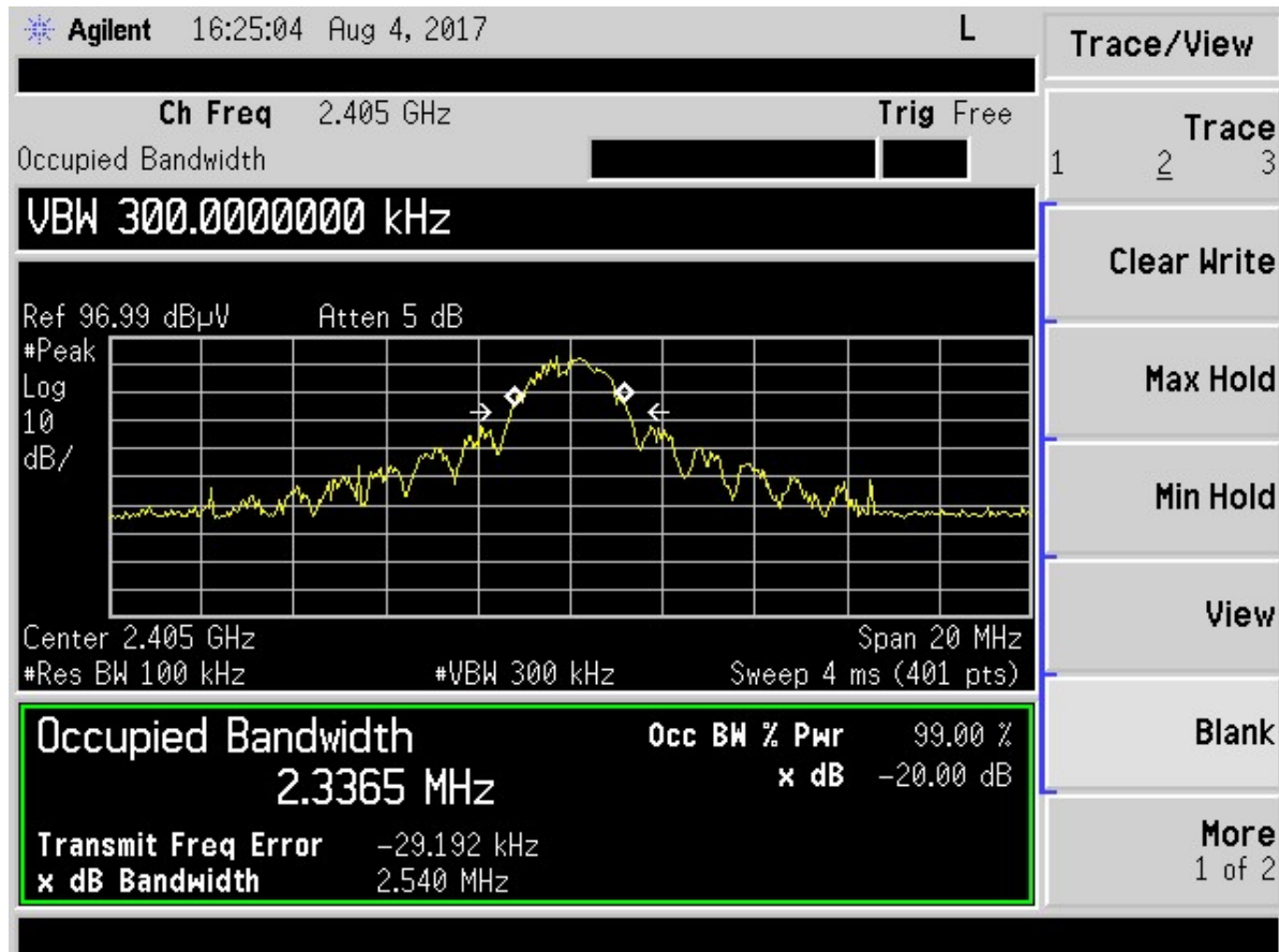
Figure 5. 99% Bandwidth – Low Channel
