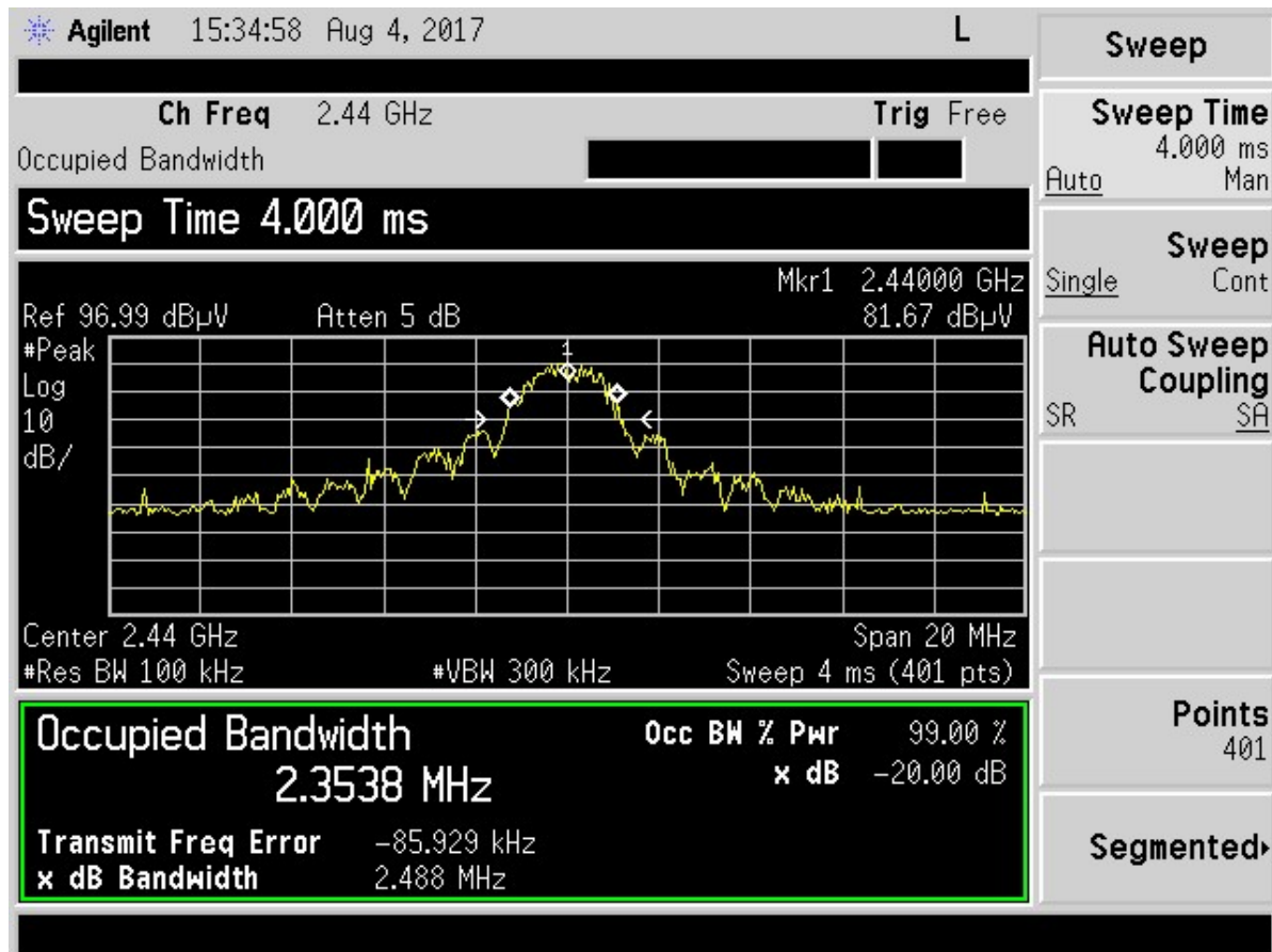
Figure 6. 99% Bandwidth – Mid Channel
