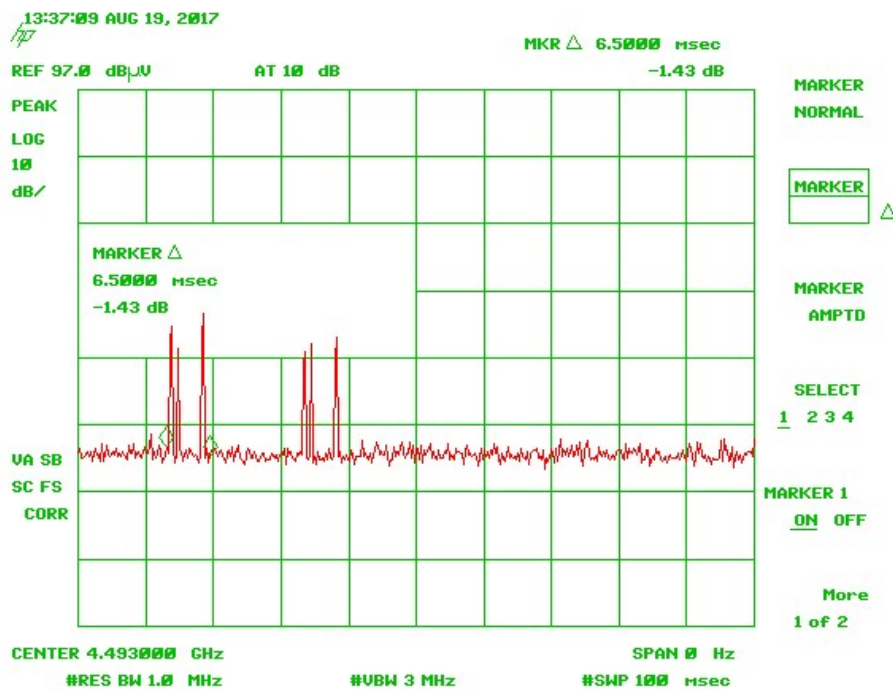
Figure 2. Measured Duty Cycle
