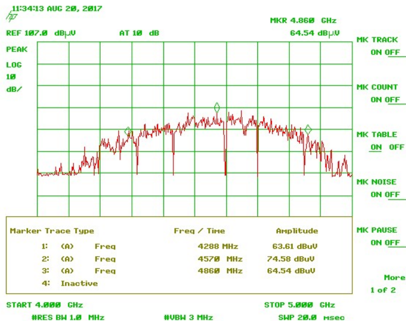
Figure 4. UWB 10 dB Bandwidth
