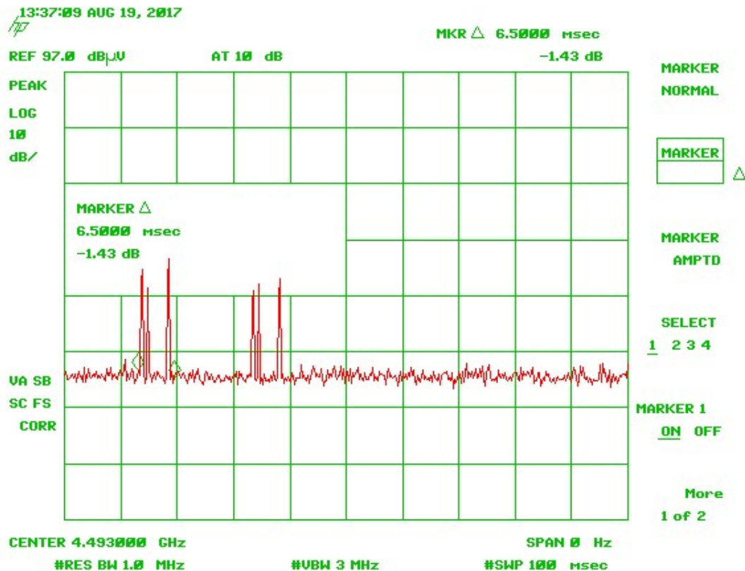
Figure 3. Pulse Repetition Frequency
