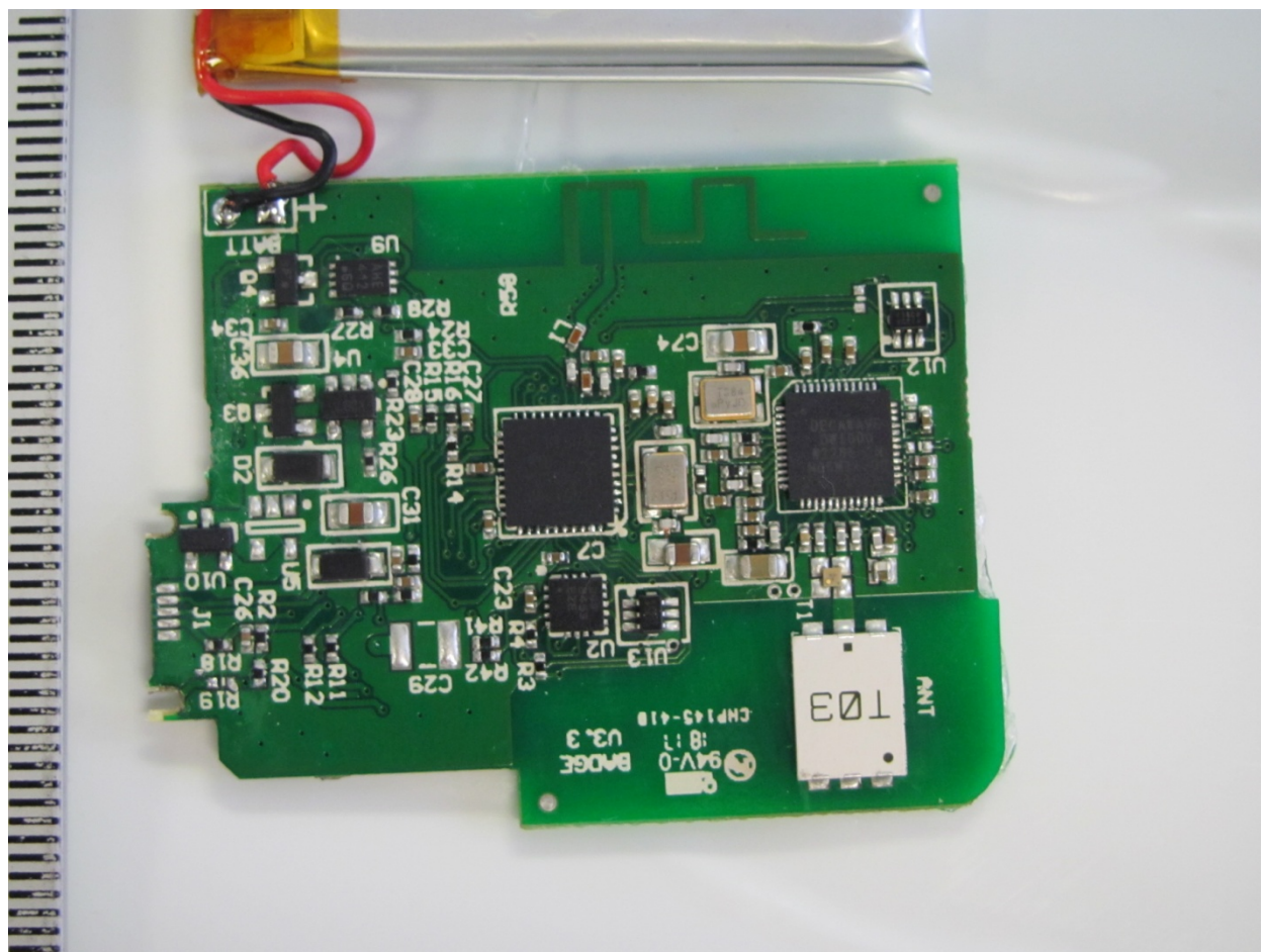
Figure 4. PCB Components
