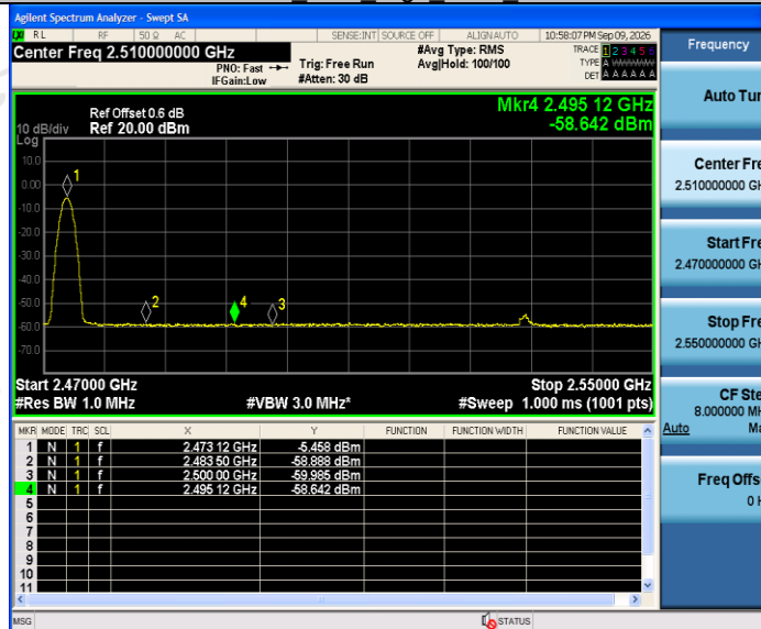
2.4G Ant1 High 2473 Peak
