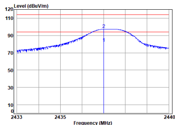
2.4G_SRD_MID_TX_Horizontal
