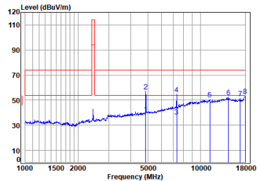
2.4G_SRD_MID_TX_Vertical
