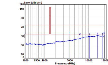
2.4G_SRD_MID_TX_Horizontal
